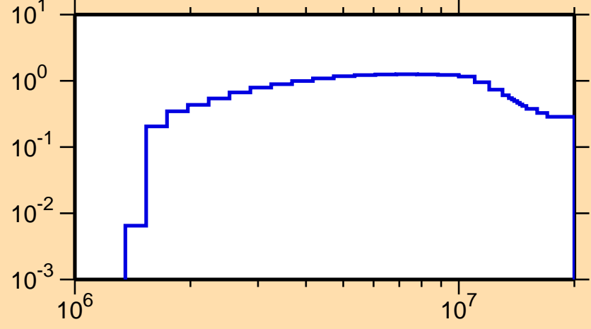
\sigma vs. E for ^{40}\text{Ar}(n,\text{inel.})
