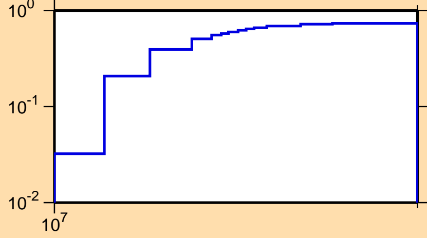
\sigma vs. E for ^{40}\text{Ar}(n,2n)
