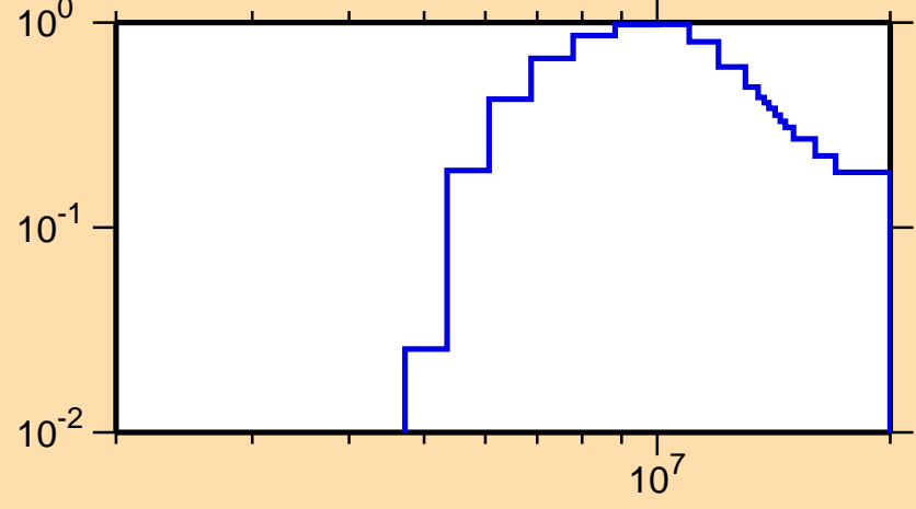
\sigma vs. E for ^{40}\text{Ar}(n,n\text{cont.})
