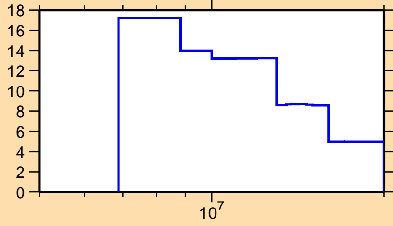
\Delta\sigma/\sigma vs. E for ^{40}\text{Ar}(n,el.)
