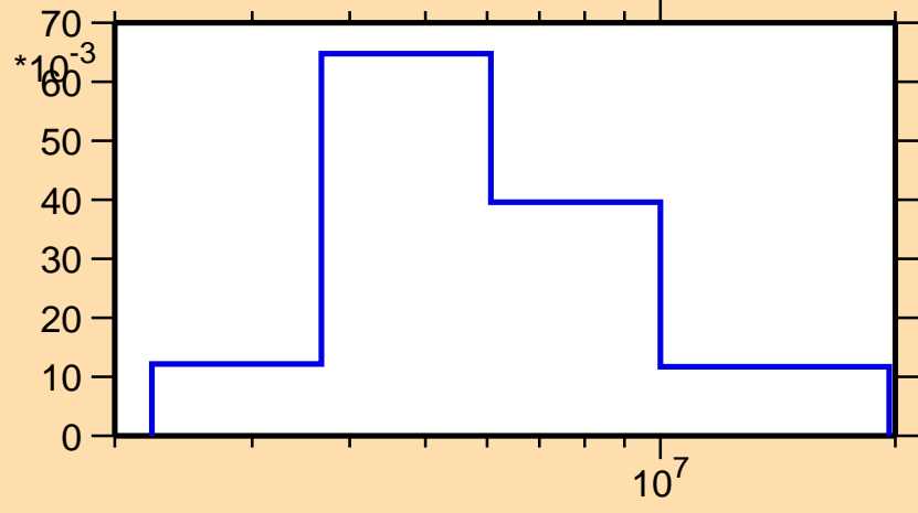
\sigma vs. E for ^{40}\text{Ar}(n,n_4)
