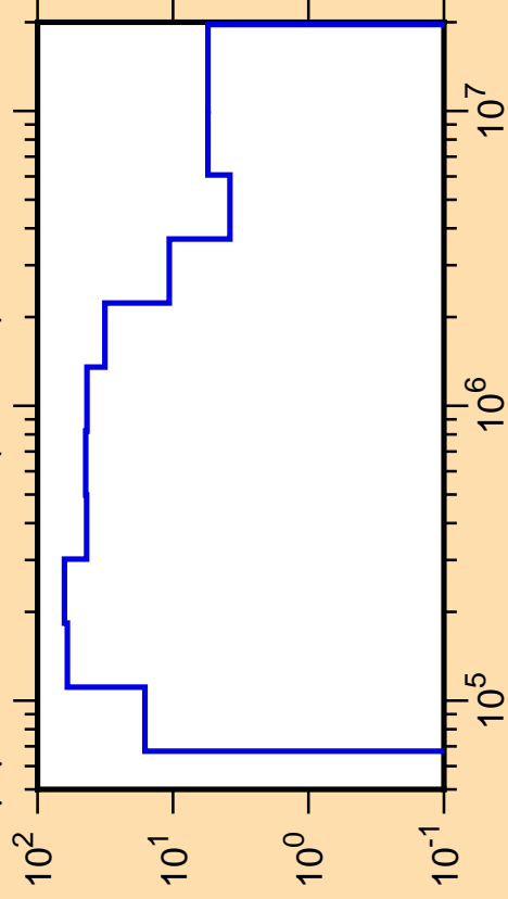
\Delta\mu/\mu vs. E for ^{42}\text{Ar}(\text{mt251})
