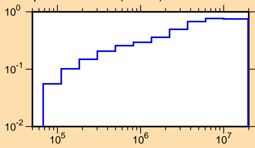
\mu vs. E for ^{42}\text{Ar}(\text{mt251})
