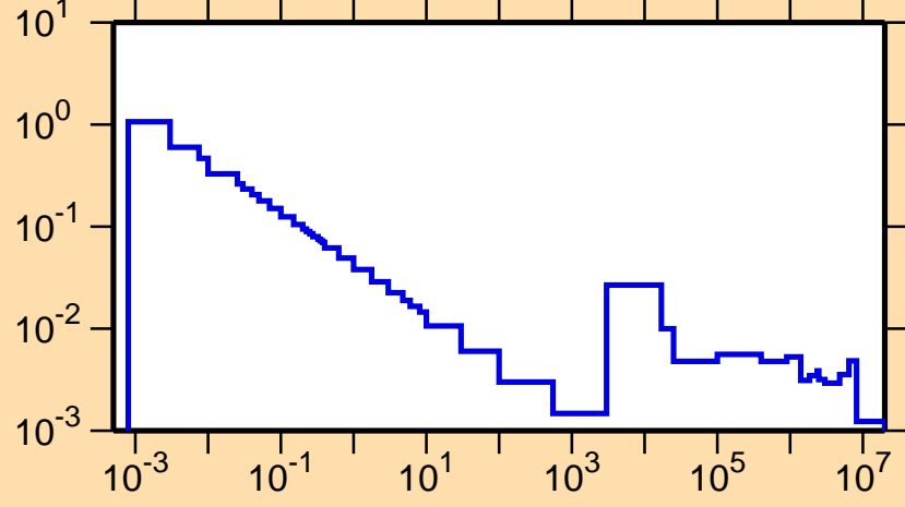
\sigma vs. E for ^{42}\text{Ar}(n,\gamma)
