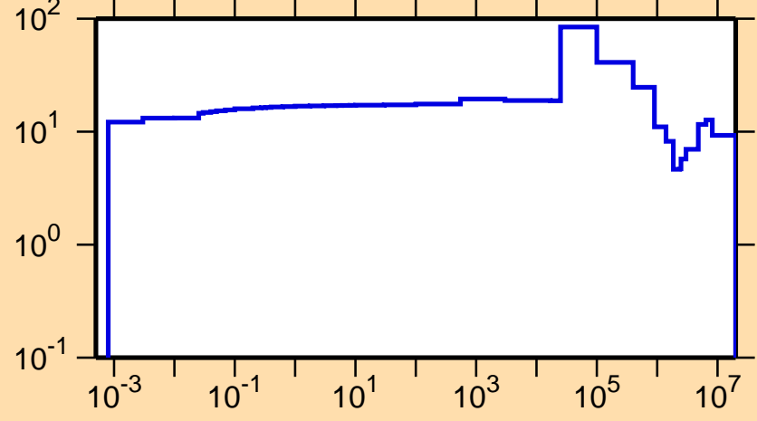
\Delta\sigma/\sigma vs. E for ^{42}\text{Ar}(n,\text{tot.})
