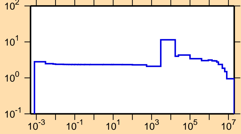
\sigma vs. E for ^{42}\text{Ar}(n,\text{el.})
