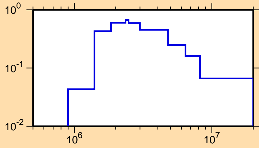
\sigma vs. E for ^{42}\text{Ar}(n,n_1)
