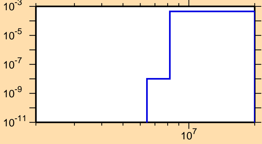
\sigma vs. E for ^{42}\text{Ar}(n,\alpha)
