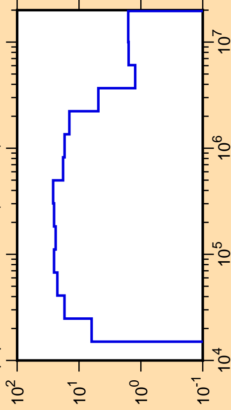
\Delta\mu/\mu vs. E for ^{43}\text{Ar}(\text{mt251})
