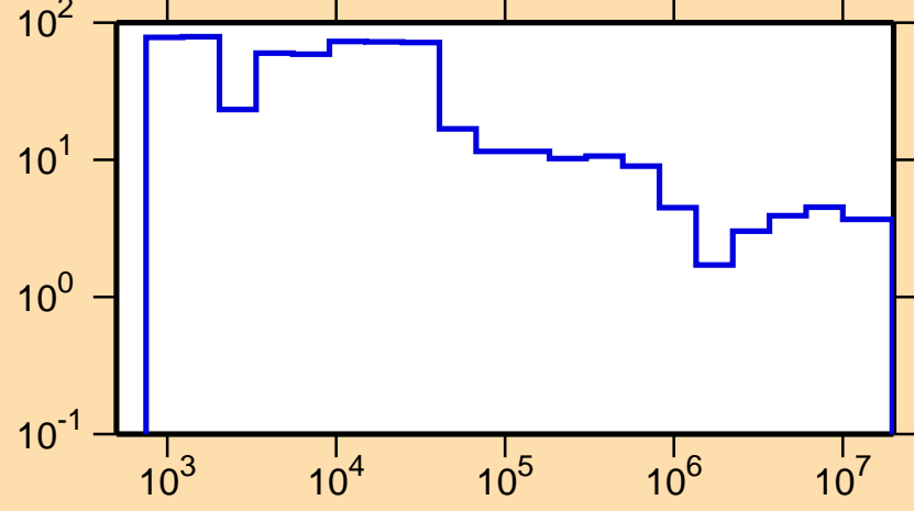
\Delta\sigma/\sigma vs. E for ^{43}\text{Ar}(n,\text{tot.})
