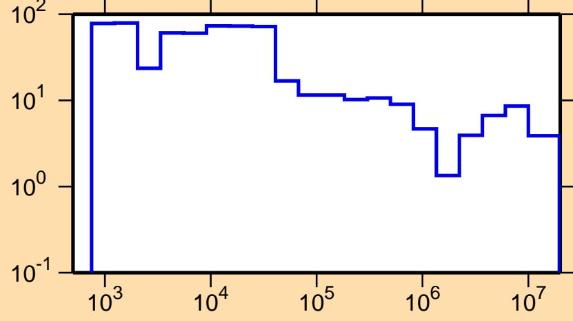
\Delta\sigma/\sigma vs. E for ^{43}\text{Ar}(n,\text{el.})
