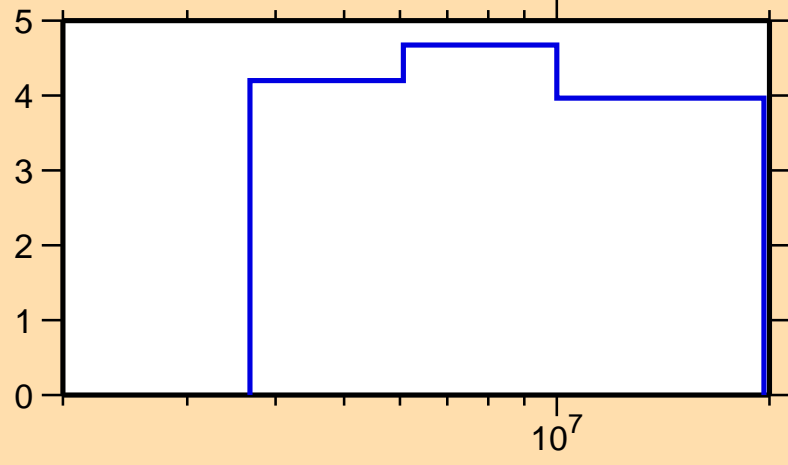
\Delta\sigma/\sigma vs. E for ^{43}\text{Ar}(n,n\text{onel.})
