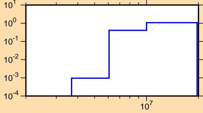
\sigma vs. E for ^{43}\text{Ar}(n,2n)
