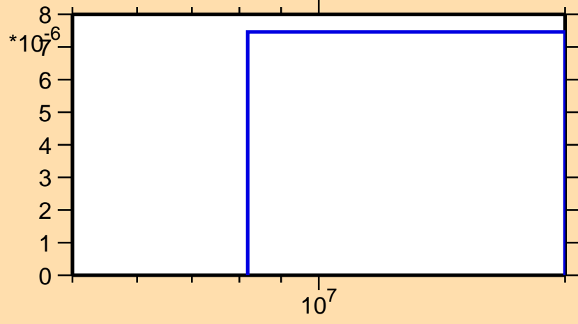
\sigma vs. E for ^{43}\text{Ar}(n,\alpha)
