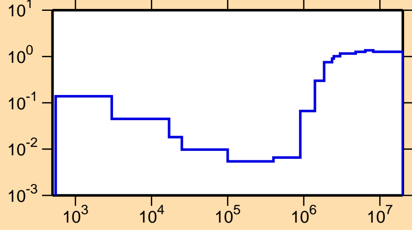
\sigma vs. E for ^{43}\text{Ar}(n,\text{nonel.})
