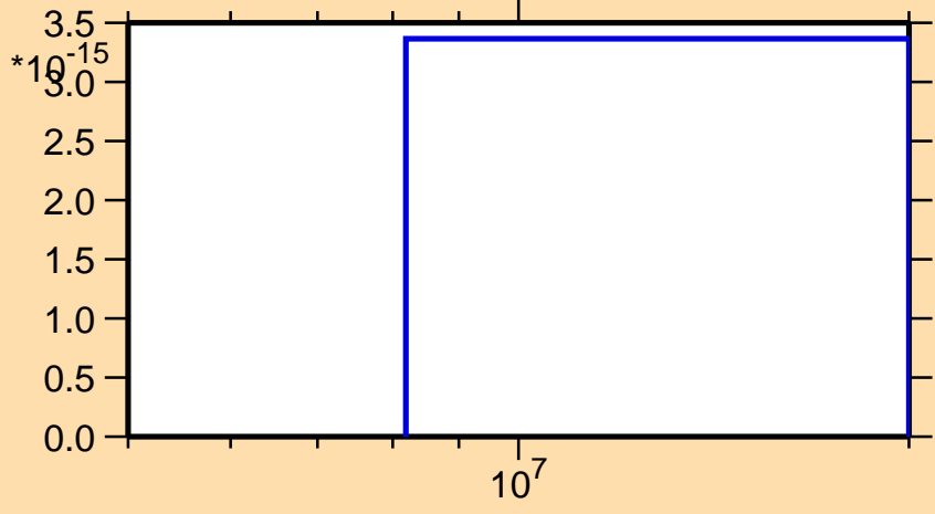
\sigma vs. E for ^{43}\text{Ar}(n,nt)
