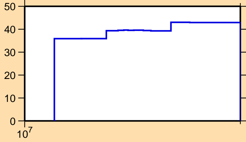
\Delta\sigma/\sigma vs. E for ^{44}\text{Ar}(n,el.)
