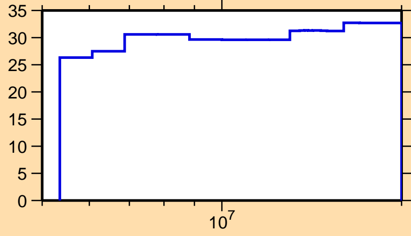
\Delta\sigma/\sigma vs. E for ^{44}\text{Ar}(n,n\text{onel.})
