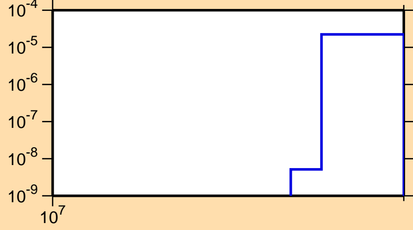
\sigma vs. E for ^{44}\text{Ar}(n,np)
