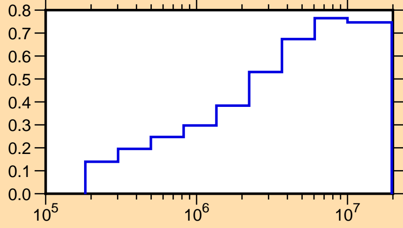
\mu vs. E for ^{44}\text{Ar}(\text{mt251})
