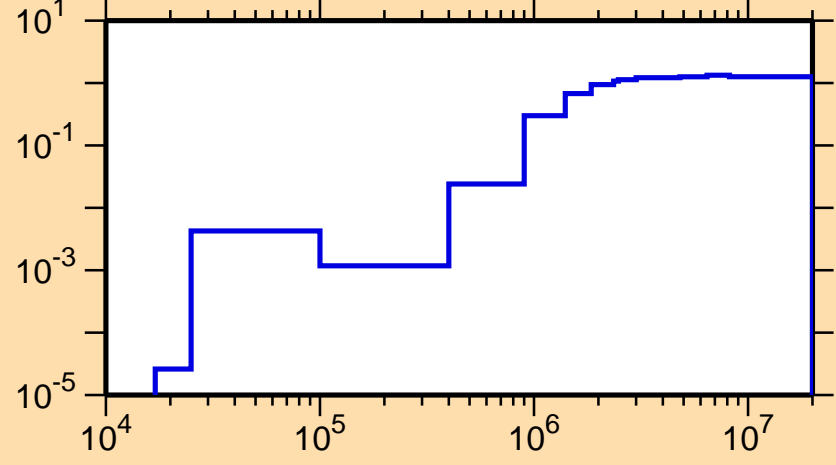
\sigma vs. E for ^{44}\text{Ar}(n,\text{nonel.})
