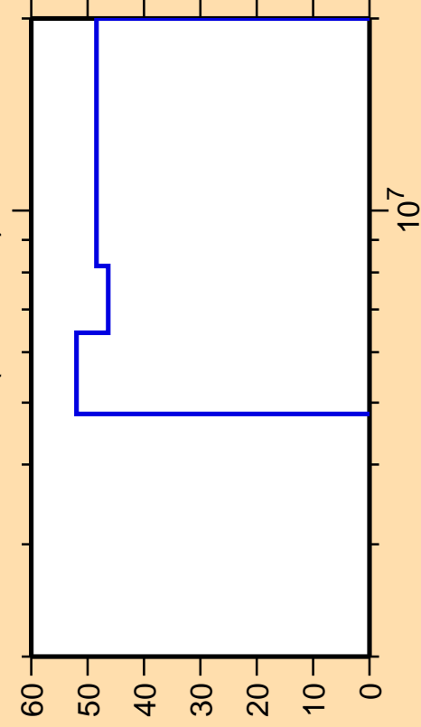
\Delta\sigma/\sigma vs. E for ^{44}\text{Ar}(n,\text{ncont.})
