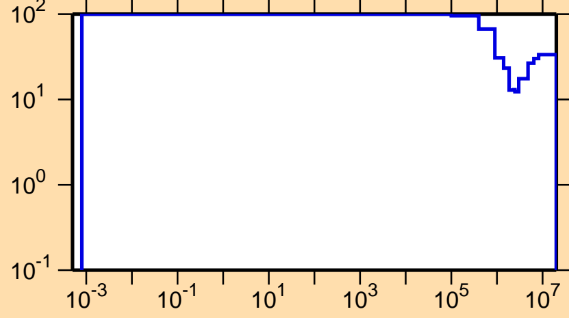
\Delta\sigma/\sigma vs. E for ^{44}\text{Ar}(n,\text{el.})
