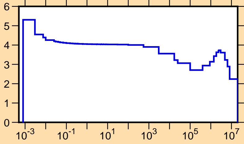
\sigma vs. E for ^{44}\text{Ar}(n,\text{tot.})
