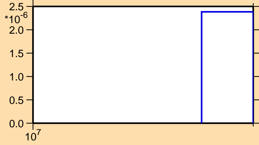
\sigma vs. E for ^{45}\text{Ar}(n,np)
