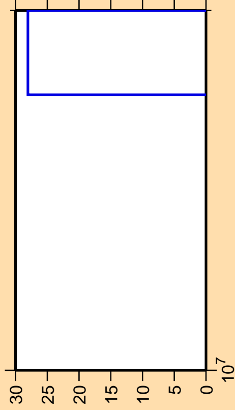
\Delta\sigma/\sigma vs. E for ^{45}\text{Ar}(n,nd)
