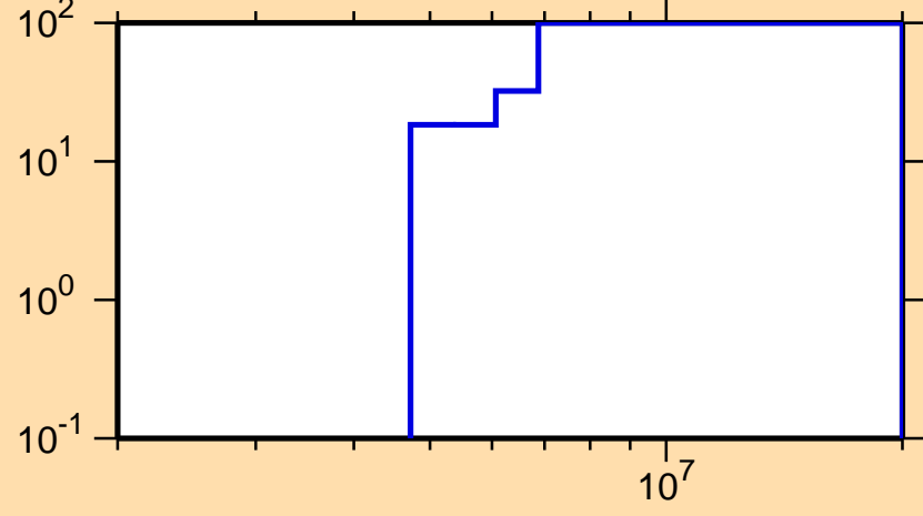
\Delta\sigma/\sigma vs. E for ^{45}\text{Ar}(n,\text{inel.})
