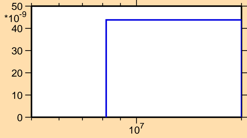
\sigma vs. E for ^{45}\text{Ar}(n,\alpha)
