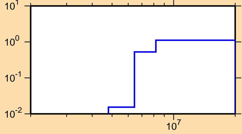
\sigma vs. E for ^{45}\text{Ar}(n,2n)
