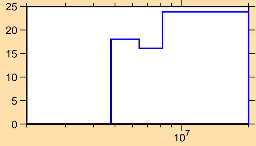
\Delta\sigma/\sigma vs. E for ^{45}\text{Ar}(n,n\text{onel.})
