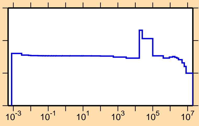
\sigma vs. E for ^{45}\text{Ar}(n,\text{el.})
