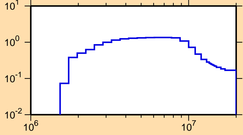
\sigma vs. E for ^{46}\text{Ar}(n,\text{inel.})
