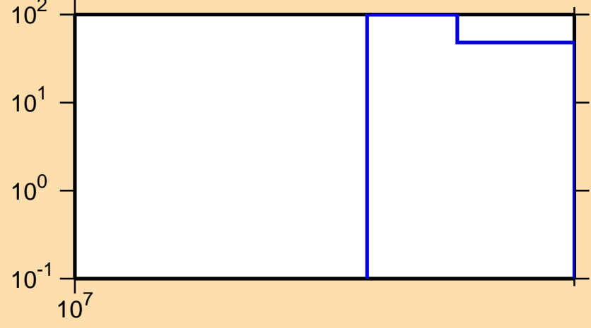
\Delta\sigma/\sigma vs. E for ^{46}\text{Ar}(n,p)
