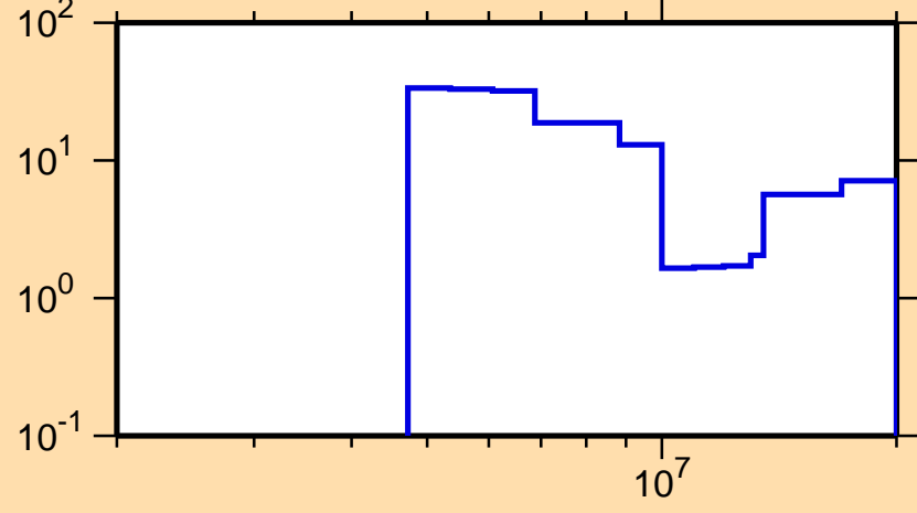
\Delta\sigma/\sigma vs. E for ^{46}\text{Ar}(n,\text{tot.})
