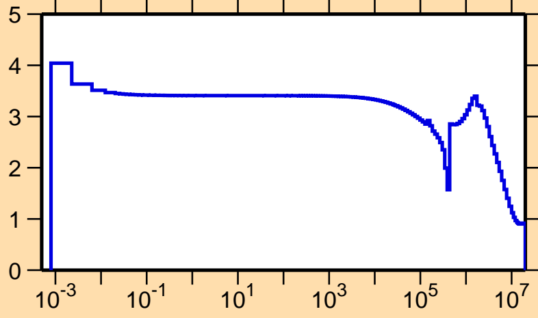
\sigma vs. E for ^{46}\text{Ar}(n,\text{el.})
