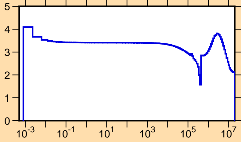
\sigma vs. E for ^{46}\text{Ar}(n,\text{tot.})
