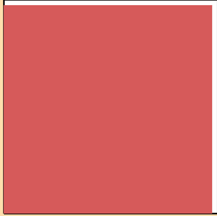
\Delta\sigma/\sigma vs. E for ^{46}\text{Ar}(n,2n)
