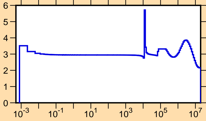
\sigma vs. E for ^{47}\text{Ar}(n,\text{tot.})
