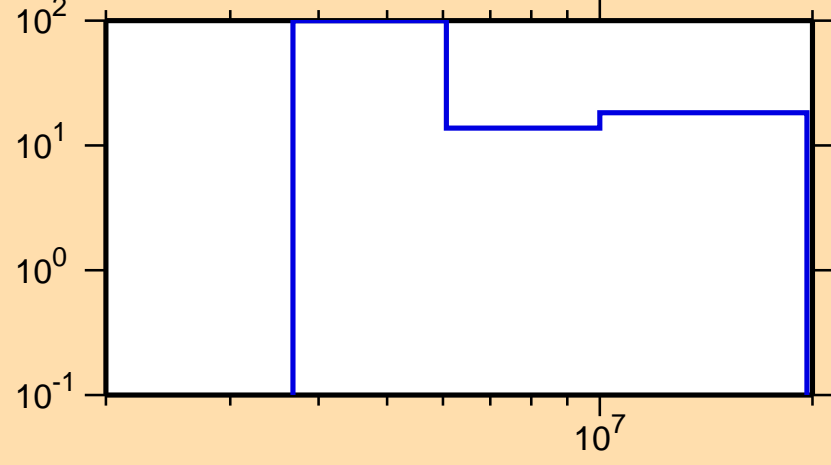
\Delta\sigma/\sigma vs. E for ^{47}\text{Ar}(n,2n)
