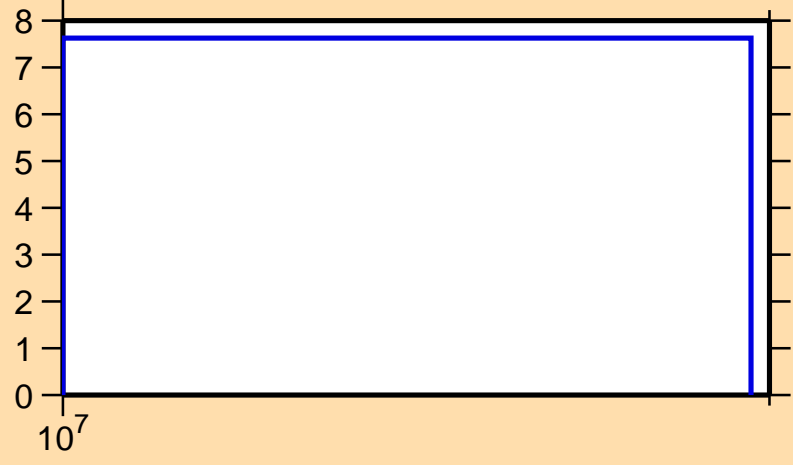
\Delta\sigma/\sigma vs. E for ^{47}\text{Ar}(n,\text{el.})
