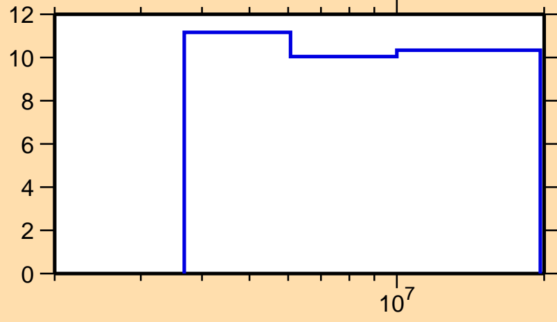
\Delta\sigma/\sigma vs. E for ^{47}\text{Ar}(n,\text{nonel.})
