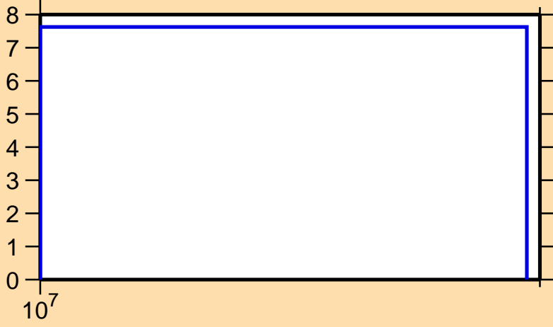
\Delta\sigma/\sigma vs. E for ^{47}\text{Ar}(n,el.)
