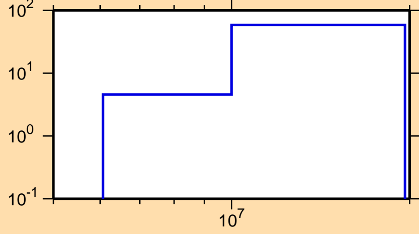
\Delta\sigma/\sigma vs. E for ^{47}\text{Ar}(n,n_1)
