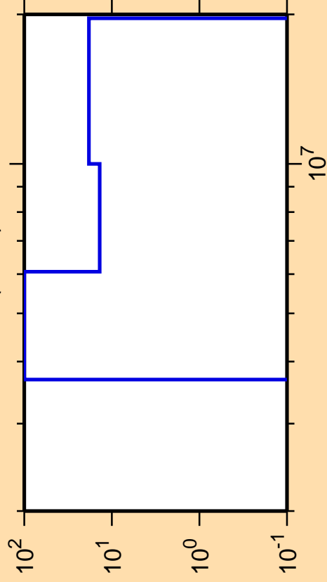
\Delta\sigma/\sigma vs. E for ^{47}\text{Ar}(n,2n)
