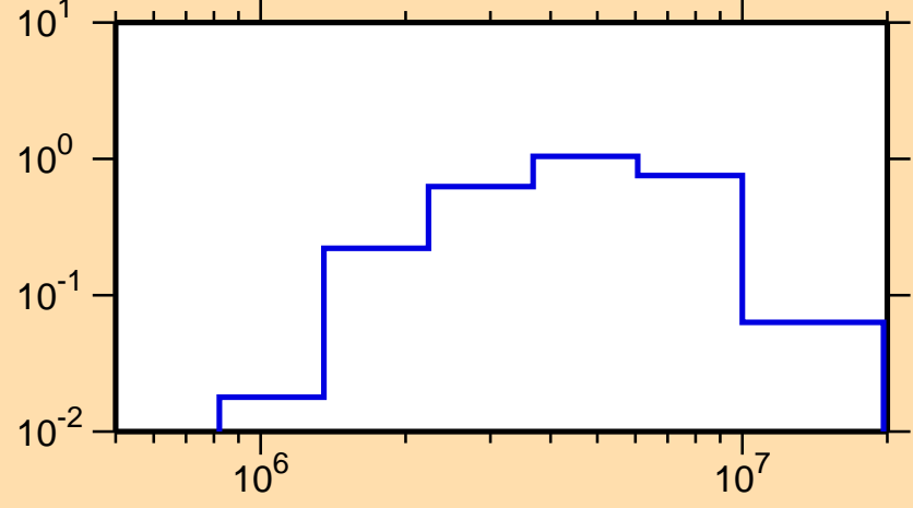
\sigma vs. E for ^{47}\text{Ar}(n,\text{inel.})
