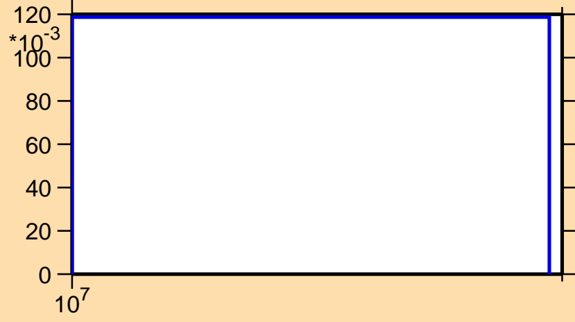
\sigma vs. E for ^{47}\text{Ar}(n,3n)
