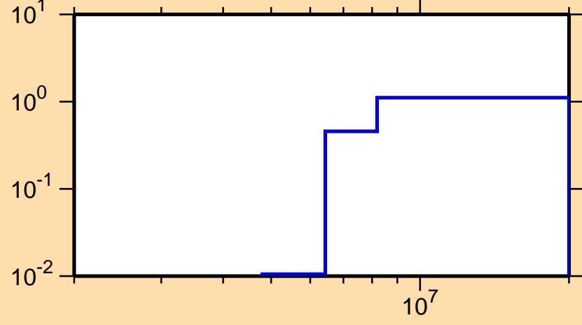
\sigma vs. E for ^{47}\text{Ar}(n,2n)
