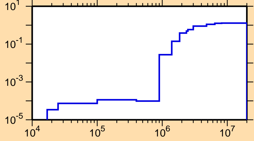
\sigma vs. E for ^{47}\text{Ar}(n,\text{nonel.})
