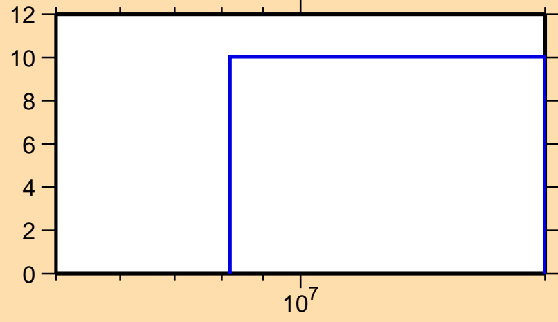
\Delta\sigma/\sigma vs. E for ^{47}\text{Ar}(n,el.)
