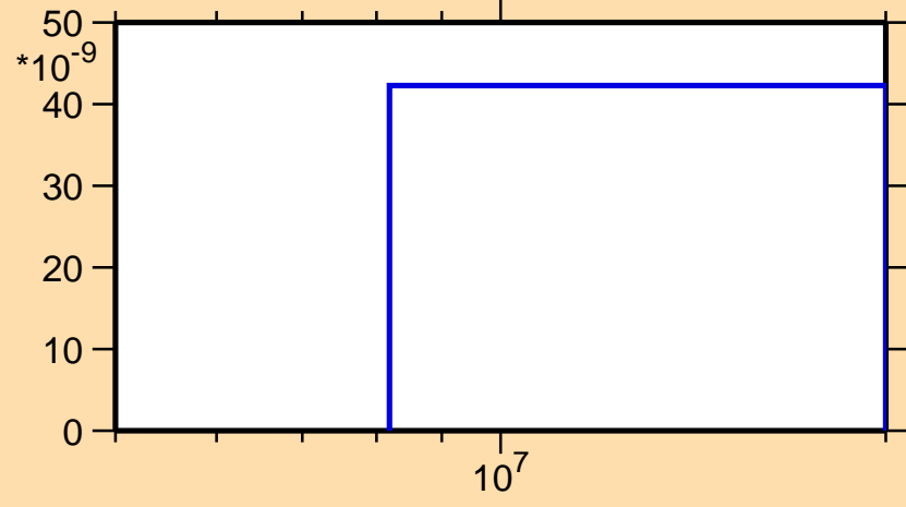
\sigma vs. E for ^{47}\text{Ar}(n,\alpha)
