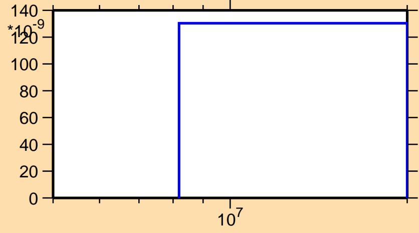
\sigma vs. E for ^{47}\text{Ar}(n,t)
