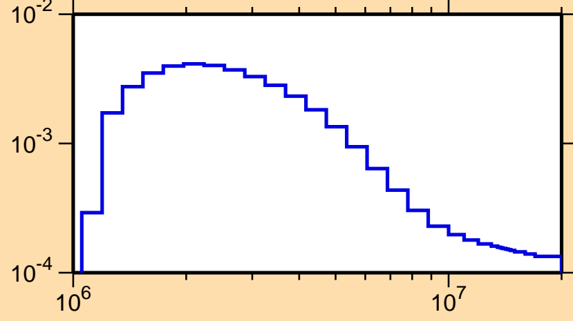
\sigma vs. E for ^{67}\text{As}(n,n_4)
