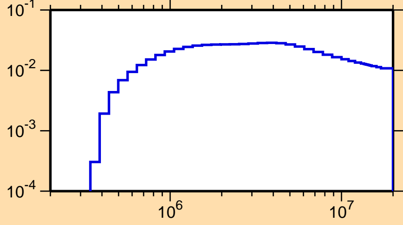
\sigma vs. E for ^{67}\text{As}(n,n_2)
