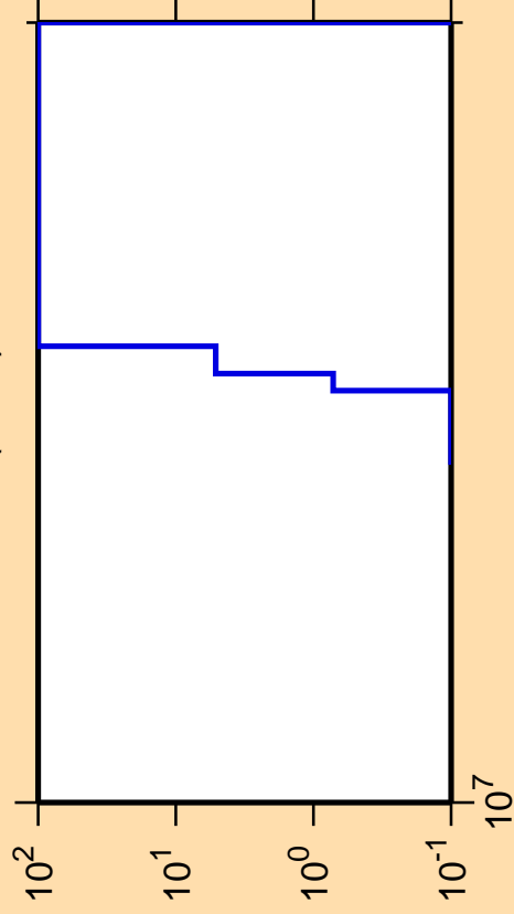
\Delta\sigma/\sigma vs. E for ^{67}\text{As}(n,nd)
