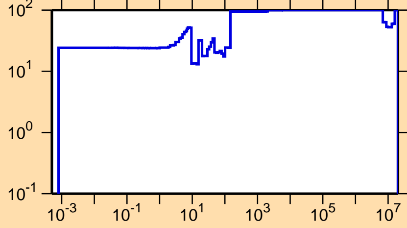
\Delta\sigma/\sigma vs. E for ^{67}\text{As}(n,\gamma)
