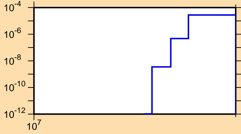
\sigma vs. E for ^{67}\text{As}(n,pt)
