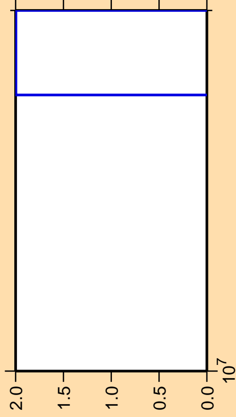
\Delta\sigma/\sigma vs. E for ^{67}\text{As}(n,nt)
