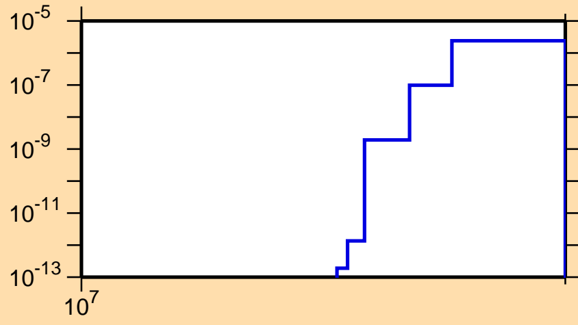
\sigma vs. E for ^{67}\text{As}(n,nd)
