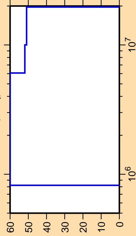
\Delta\sigma/\sigma vs. E for ^{67}\text{As}(n,n_4)
