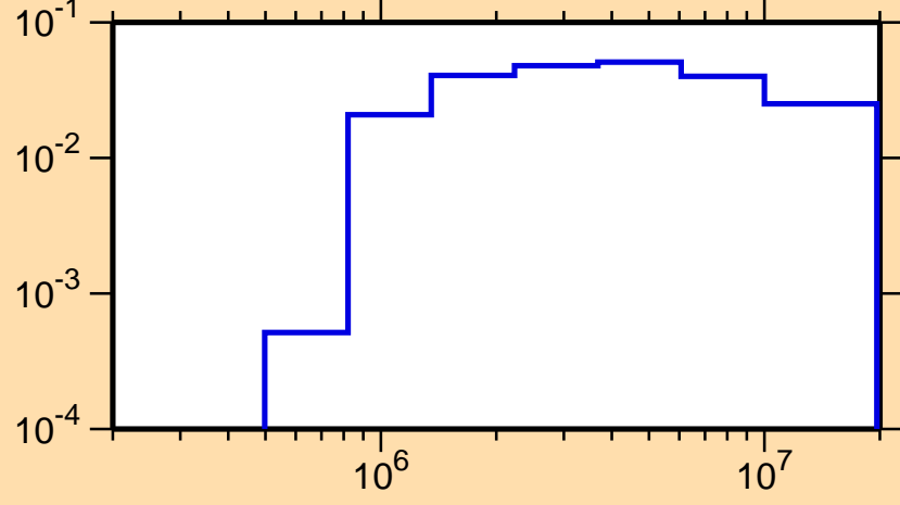
\sigma vs. E for ^{67}\text{As}(n,n_3)
