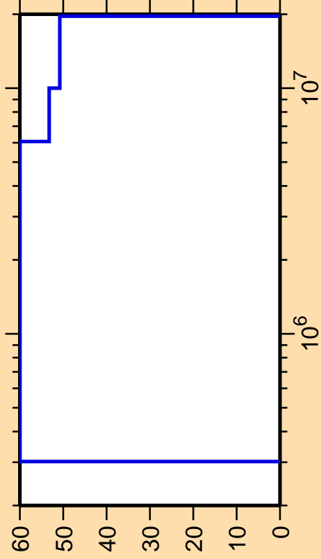
\Delta\sigma/\sigma vs. E for ^{67}\text{As}(n,n_2)
