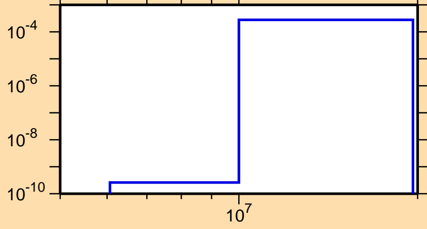
\sigma vs. E for ^{67}\text{As}(n,t)
