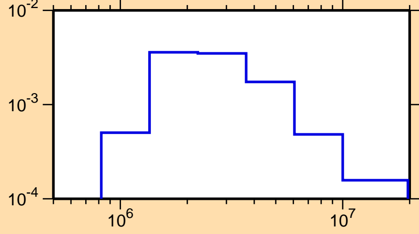
\sigma vs. E for ^{67}\text{As}(n,n_4)
