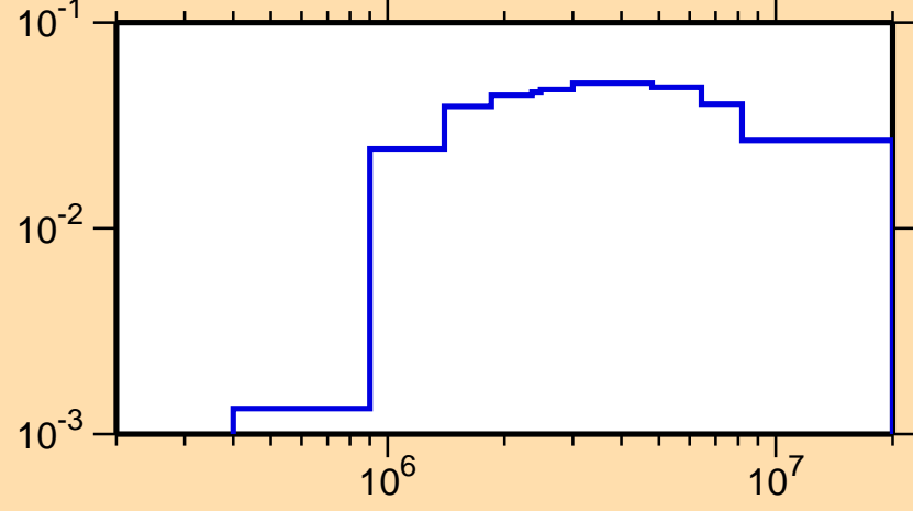
\sigma vs. E for ^{67}\text{As}(n,n_3)
