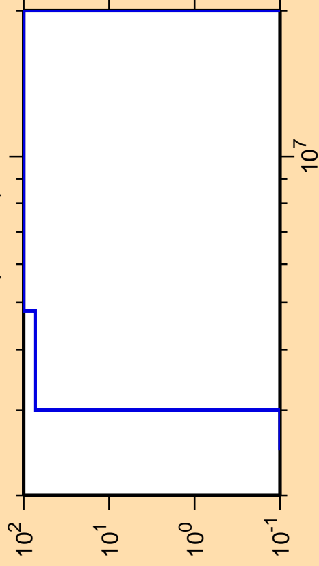
\Delta\sigma/\sigma vs. E for ^{67}\text{As}(n,\text{He3})
