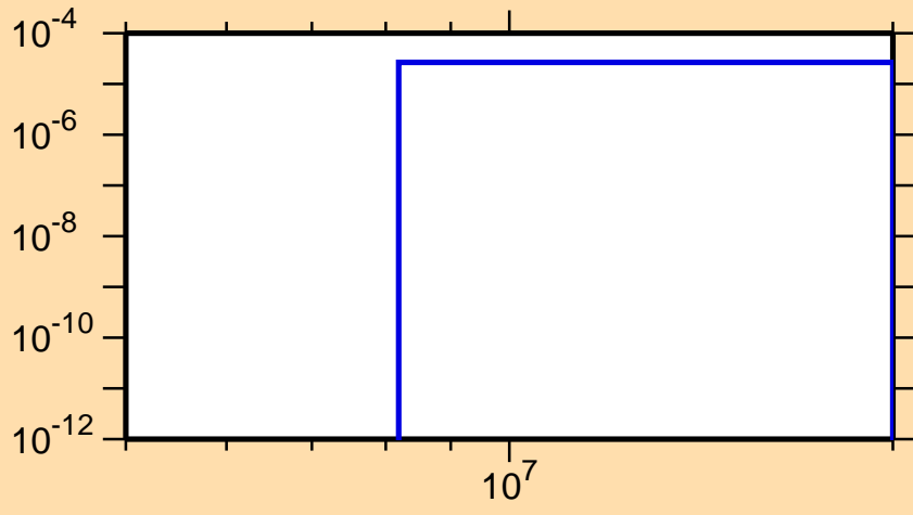
\sigma vs. E for ^{67}\text{As}(\text{mt117})
