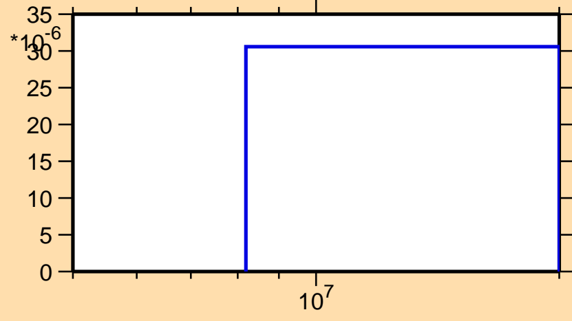
\sigma vs. E for ^{67}\text{As}(n,2n)
