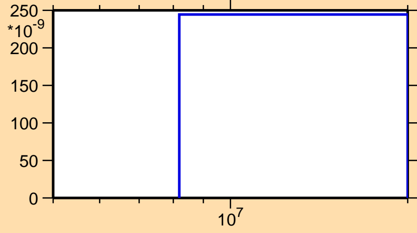
\sigma vs. E for ^{67}\text{As}(n,\text{pt})
