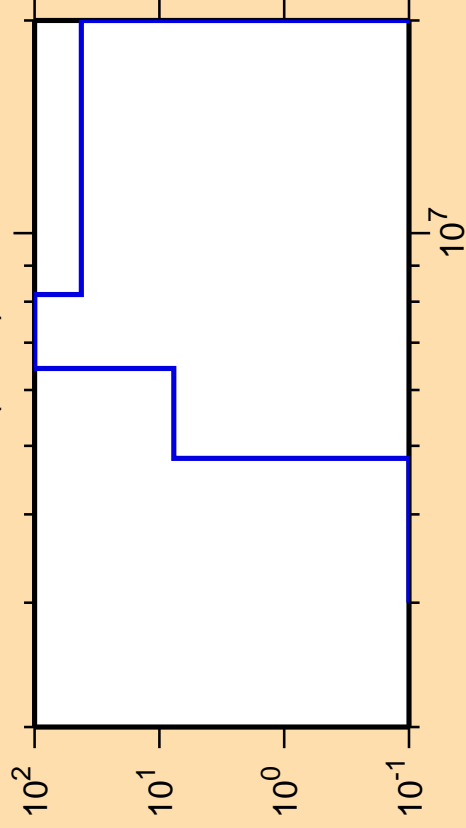
\Delta\sigma/\sigma vs. E for ^{67}\text{As}(n,n\alpha)
