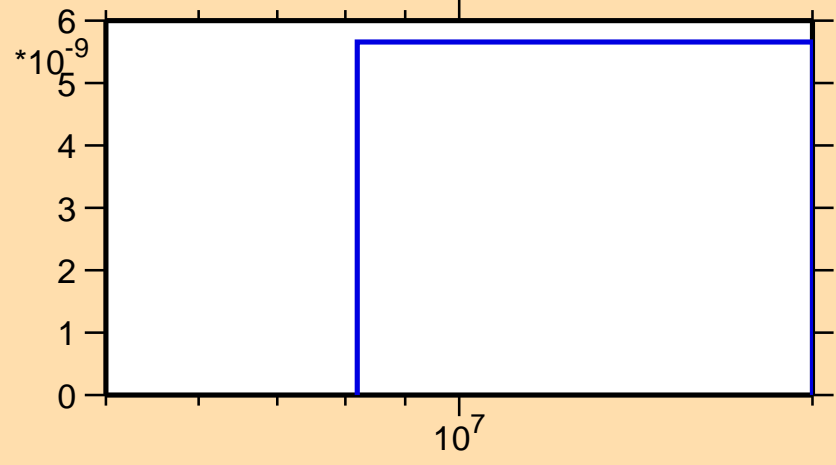
\sigma vs. E for ^{67}\text{As}(n,2np)
