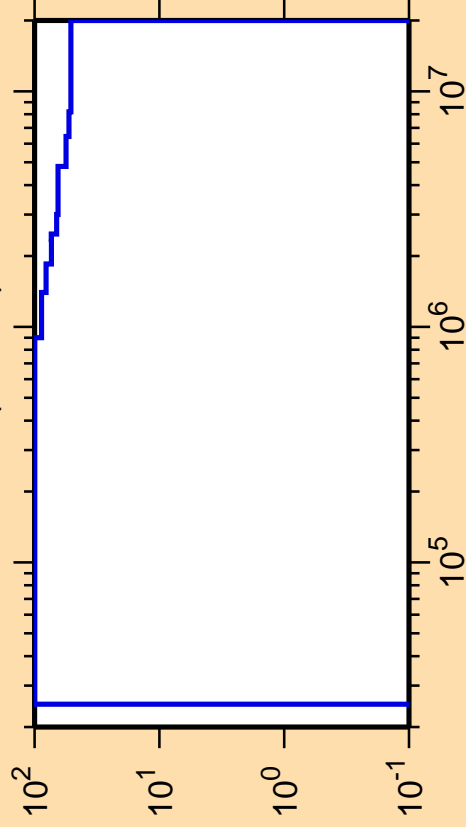
\Delta\sigma/\sigma vs. E for ^{67}\text{As}(n,\text{inel.})
