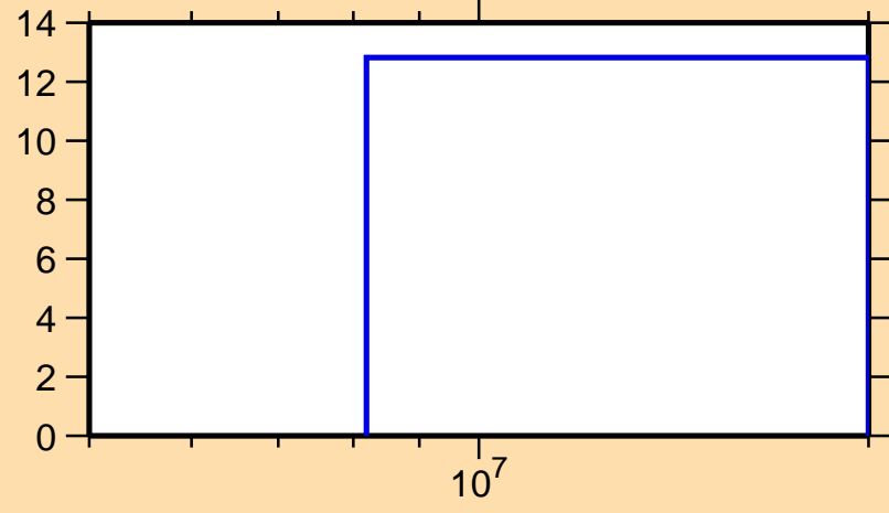
\Delta\sigma/\sigma vs. E for ^{67}\text{As}(n,\text{el.})
