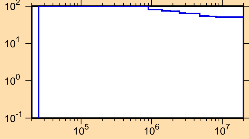
\Delta\sigma/\sigma vs. E for ^{67}\text{As}(n,n_1)
