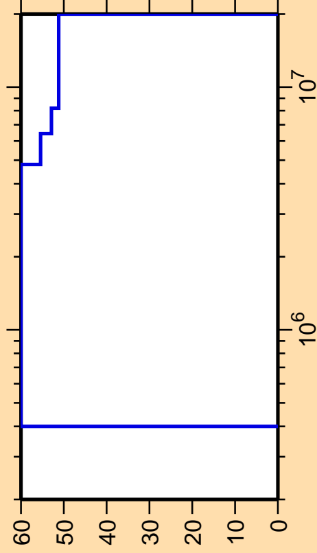
\Delta\sigma/\sigma vs. E for ^{67}\text{As}(n,n_3)
