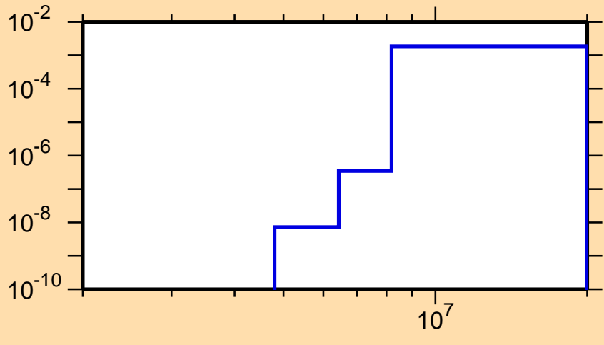
\sigma vs. E for ^{67}\text{As}(n,\text{He3})
