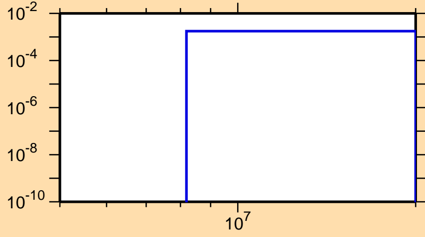
\sigma vs. E for ^{67}\text{As}(n,pd)
