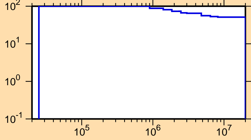
\Delta\sigma/\sigma vs. E for ^{67}\text{As}(n,\text{inel.})
