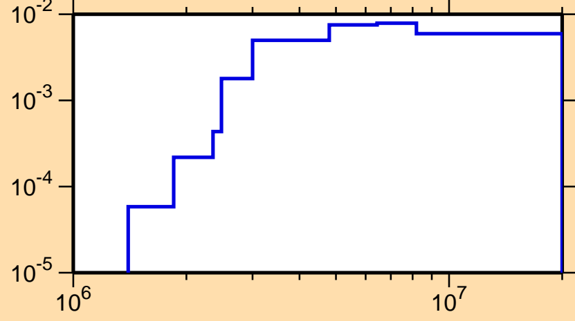
\sigma vs. E for ^{67}\text{As}(n,n\text{cont.})
