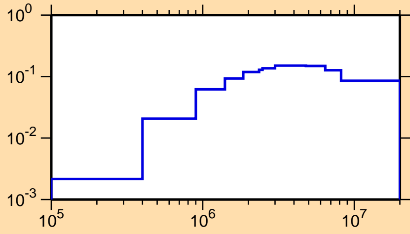
\sigma vs. E for ^{67}\text{As}(n,\text{inel.})
