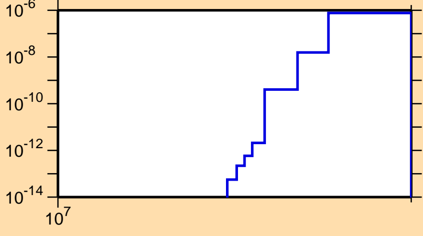
\sigma vs. E for ^{68}\text{As} (mt 34)
