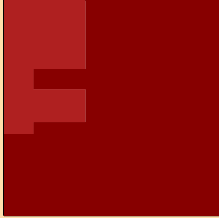
\Delta\sigma/\sigma vs. E for ^{68}\text{As}(n,2n)
