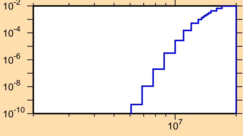
\sigma vs. E for ^{68}\text{As}(n,\text{He3})
