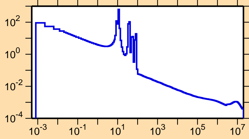
\sigma vs. E for ^{68}\text{As}(n,\gamma)
