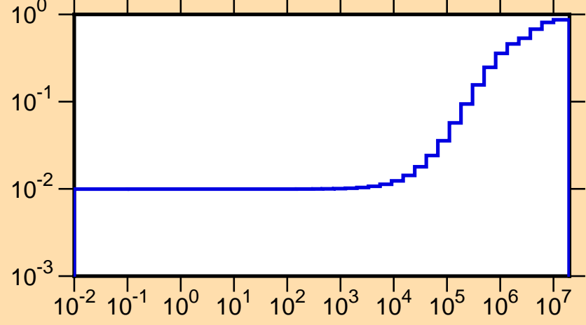
\mu vs. E for ^{68}\text{As}(\text{mt251})
