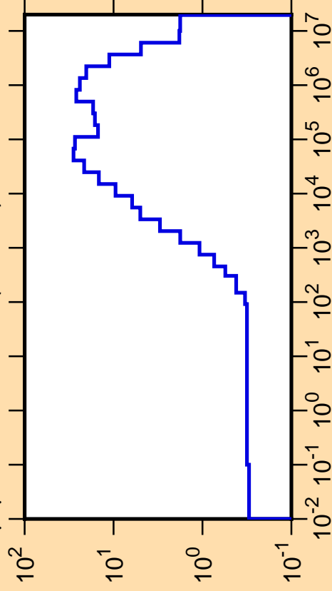
\Delta\mu/\mu vs. E for ^{68}\text{As}(\text{mt251})
