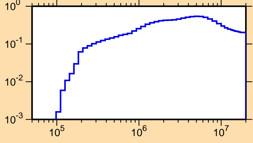
\sigma vs. E for ^{69}\text{As}(n,\text{inel.})
