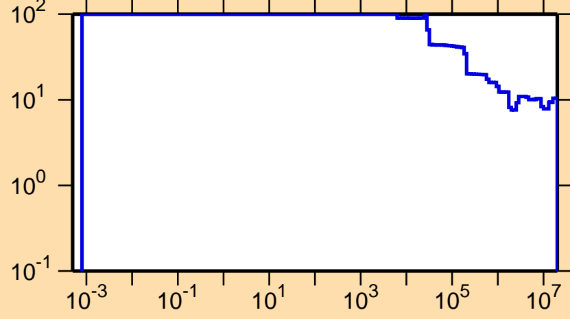
\Delta\sigma/\sigma vs. E for ^{69}\text{As}(n,\text{nonel.})
