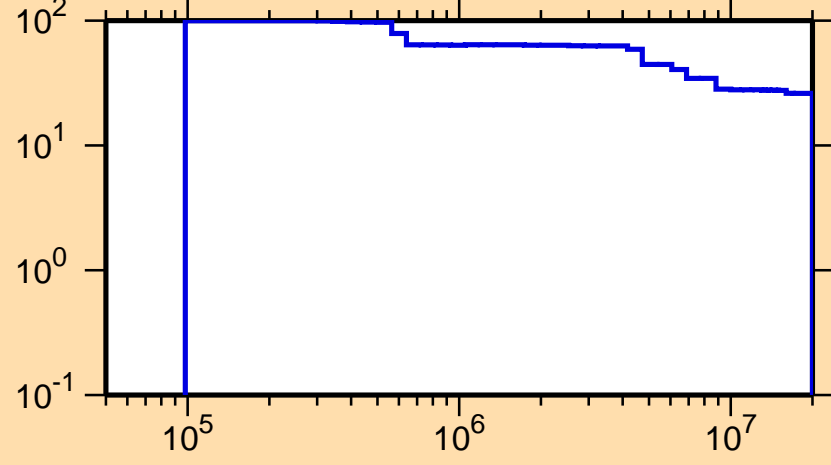
\Delta\sigma/\sigma vs. E for ^{69}\text{As}(n,\text{inel.})
