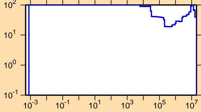
\Delta\sigma/\sigma vs. E for ^{69}\text{As}(n,p)
