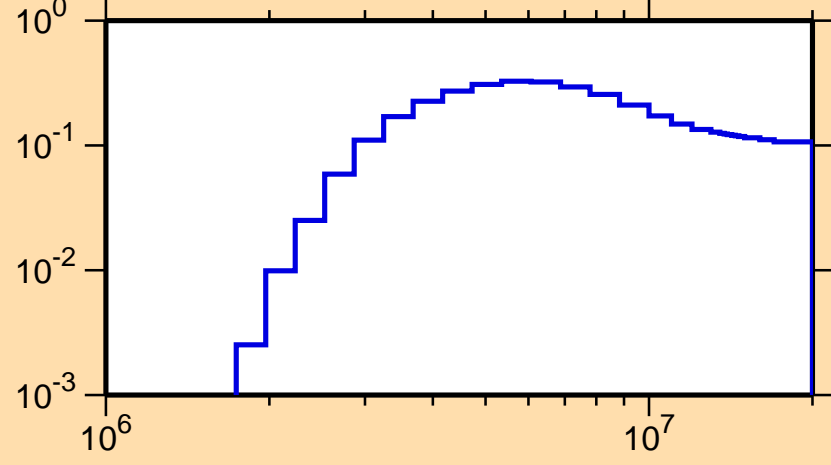
\sigma vs. E for ^{69}\text{As}(n,n\text{cont.})
