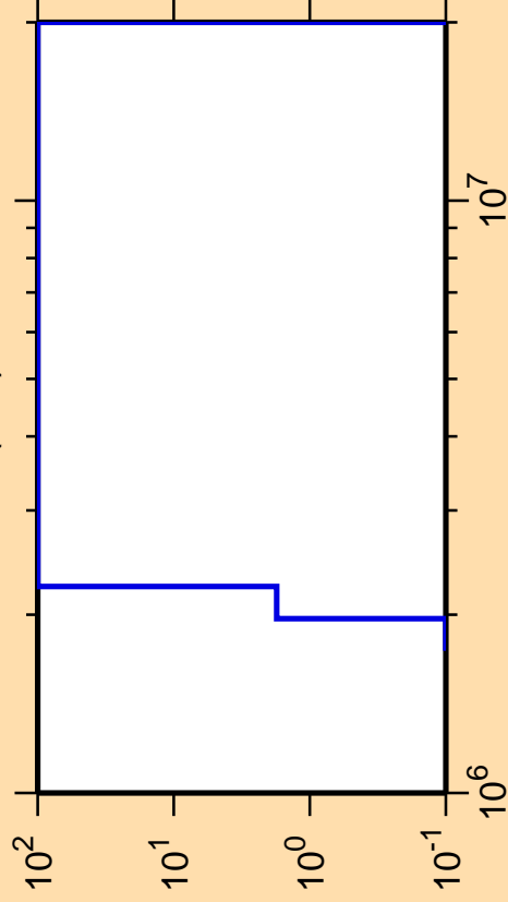
\Delta\sigma/\sigma vs. E for ^{69}\text{As}(n,d)
