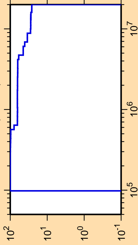
\Delta\sigma/\sigma vs. E for ^{69}\text{As}(n,\text{inel.})
