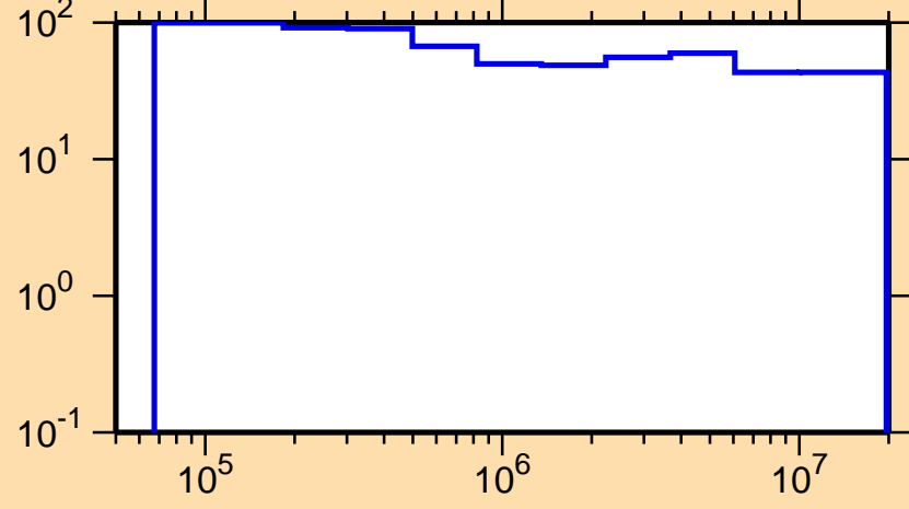
\Delta\sigma/\sigma vs. E for ^{69}\text{As}(n,n_1)
