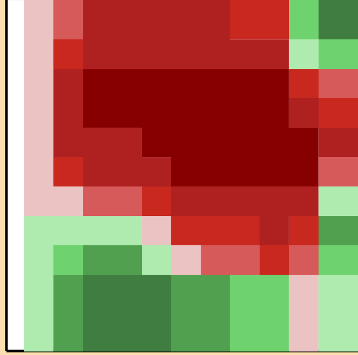
\Delta\sigma/\sigma vs. E for ^{69}\text{As}(n,\text{inel.})
