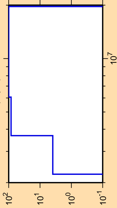
\Delta\sigma/\sigma vs. E for ^{69}\text{As}(n,p\alpha)
