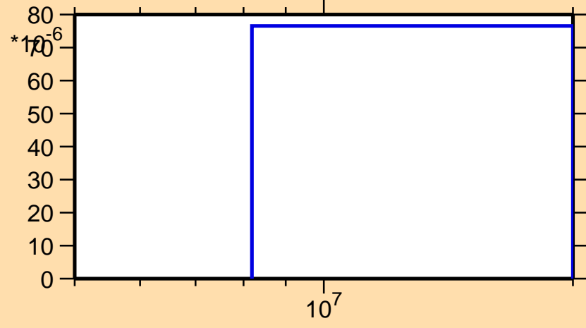
\sigma vs. E for ^{69}\text{As}(n,pd)
