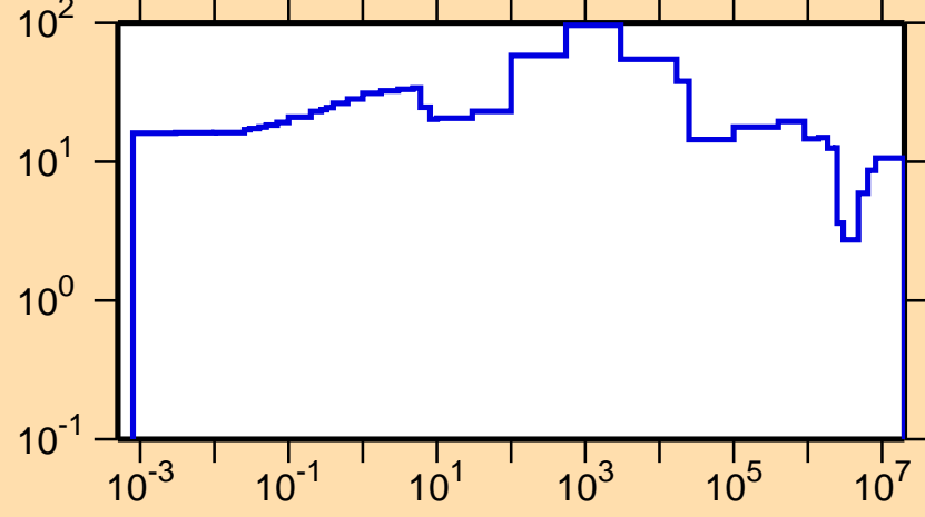
\Delta\sigma/\sigma vs. E for ^{69}\text{As}(n,\text{tot.})
