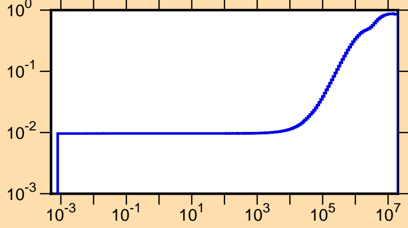
\mu vs. E for ^{70}\text{As}(\text{mt251})
