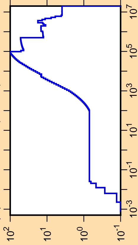
\Delta\mu/\mu vs. E for ^{70}\text{As}(\text{mt251})
