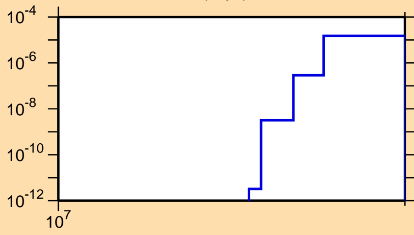
\sigma vs. E for ^{70}\text{As}(n,pt)
