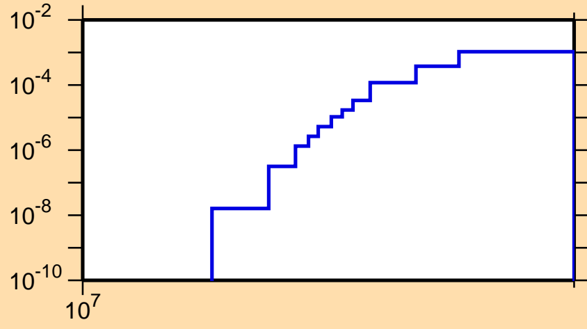
\sigma vs. E for ^{70}\text{As}(n,\text{nd})
