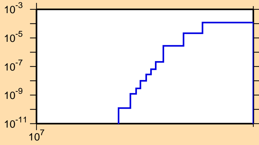
\sigma vs. E for ^{70}\text{As}(n,pd)
