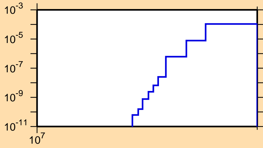
\sigma vs. E for ^{70}\text{As} (mt 45)
