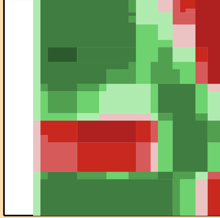
\Delta\sigma/\sigma vs. E for ^{70}\text{As}(n,n\text{cont.})
