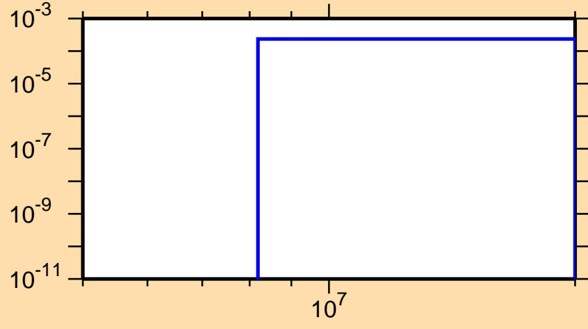
\sigma vs. E for ^{70}\text{As}(n,\text{He3})
