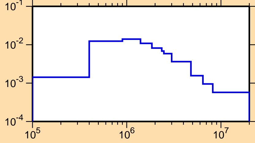
\sigma vs. E for ^{70}\text{As}(n,n_4)
