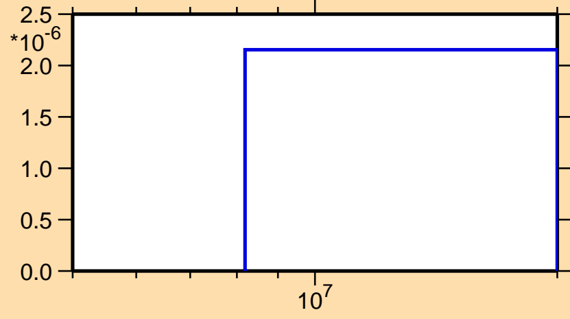
\sigma vs. E for ^{70}\text{As}(n,pd)
