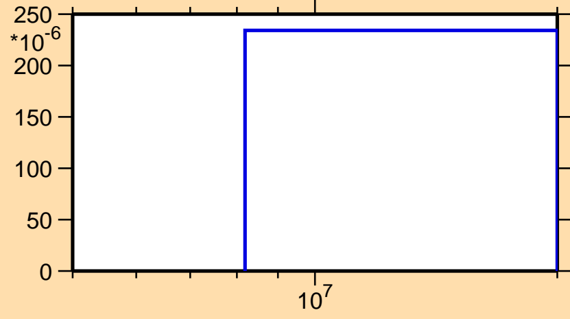
\sigma vs. E for ^{70}\text{As}(n,2np)
