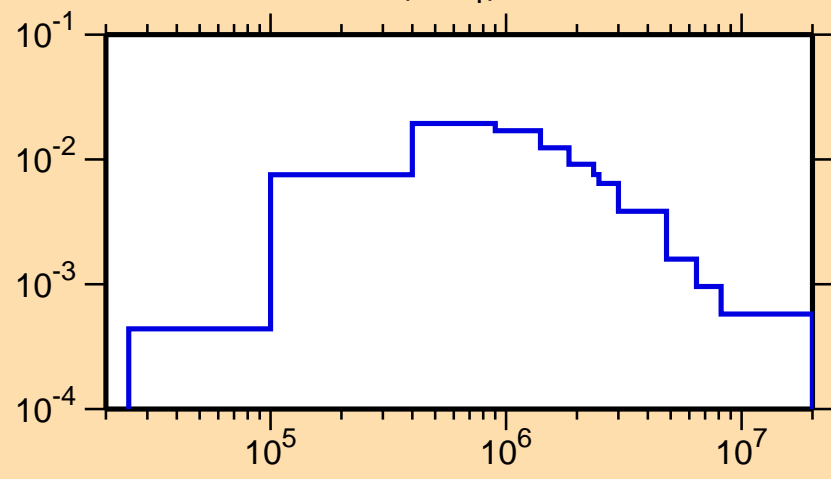
\sigma vs. E for ^{70}\text{As}(n,n_1)
