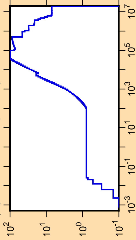
\Delta\mu/\mu vs. E for ^{72}\text{As}(\text{mt251})
