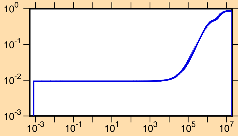
\mu vs. E for ^{72}\text{As}(\text{mt251})
