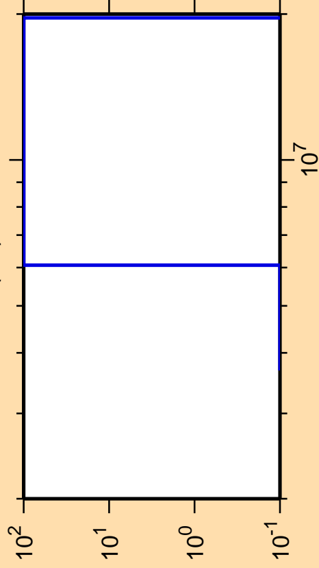
\Delta\sigma/\sigma vs. E for ^{72}\text{As}(n,t)
