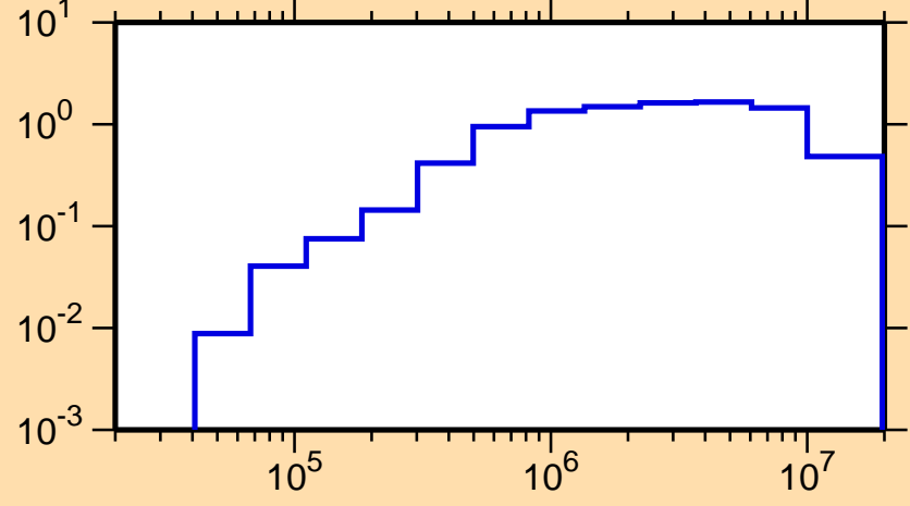
\sigma vs. E for ^{72}\text{As}(n,\text{inel.})
