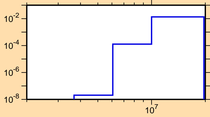
\sigma vs. E for ^{72}\text{As}(n,d)
