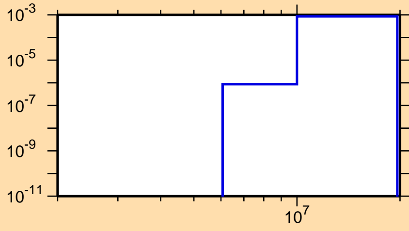
\sigma vs. E for ^{72}\text{As}(n,t)
