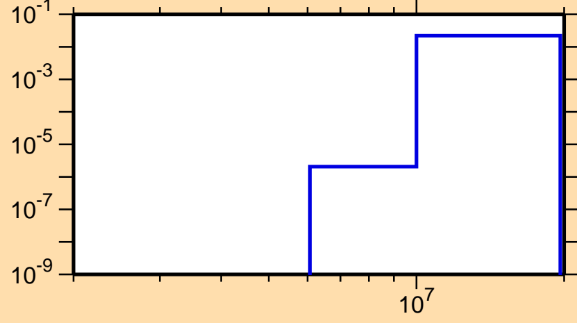
\sigma vs. E for ^{72}\text{As}(n,n\alpha)
