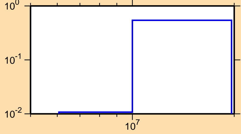
\sigma vs. E for ^{72}\text{As}(n,2n)
