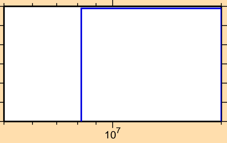
\sigma vs. E for ^{72}\text{As}(\text{mt117})
