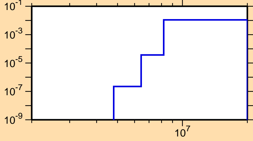
\sigma vs. E for ^{72}\text{As}(n,d)
