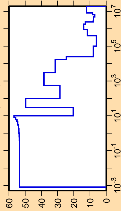
\Delta\sigma/\sigma vs. E for ^{73}\text{As}(n,\text{el.})
