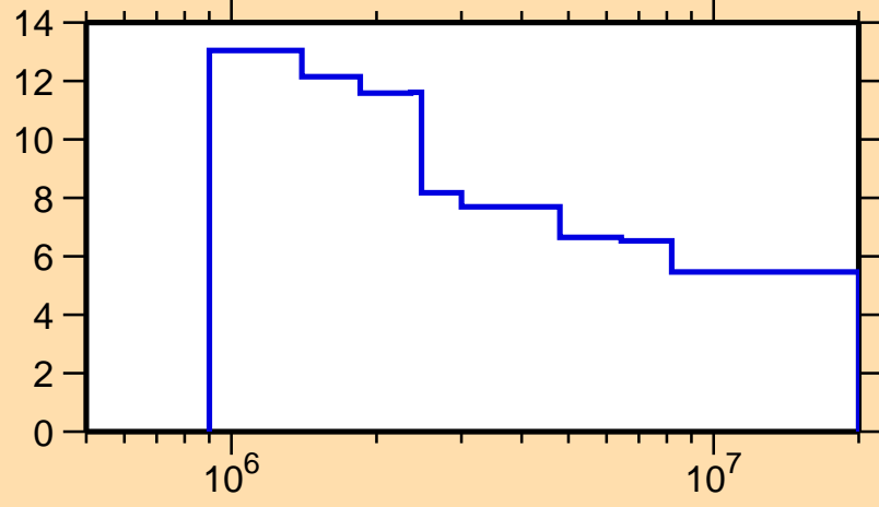
\Delta\sigma/\sigma vs. E for ^{73}\text{As}(n,n\text{onel.})
