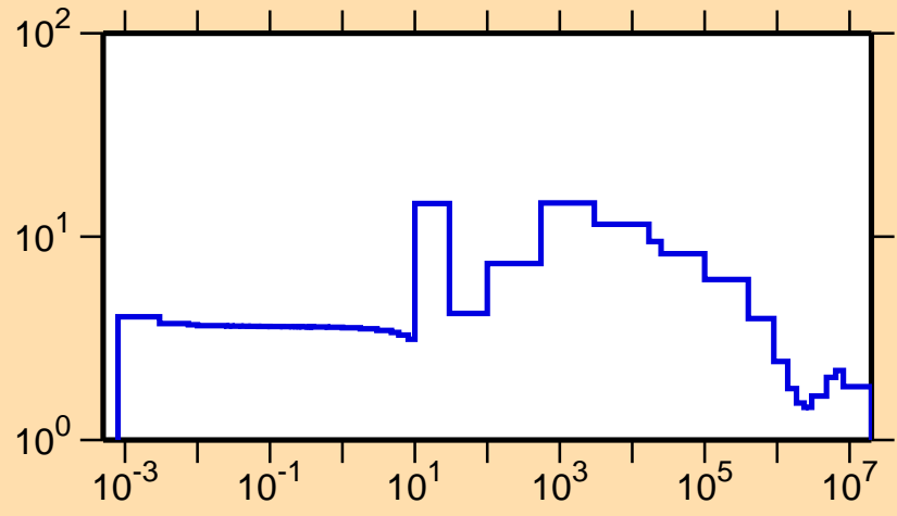
\sigma vs. E for ^{73}\text{As}(n,\text{el.})
