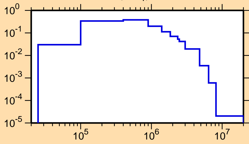
\sigma vs. E for ^{73}\text{As}(n,n_1)
