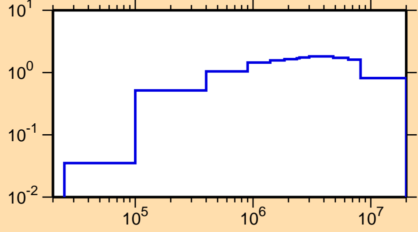
\sigma vs. E for ^{73}\text{As}(n,\text{inel.})
