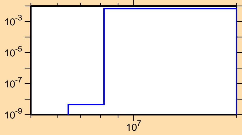
\sigma vs. E for ^{73}\text{As}(n,\alpha)
