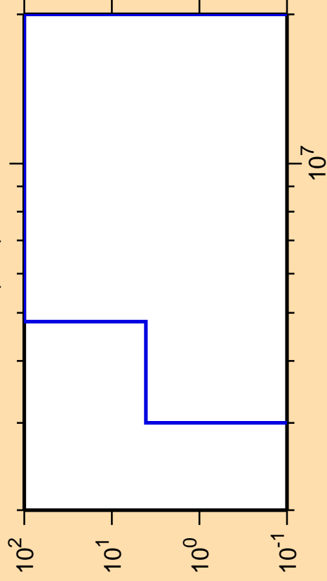
\Delta\sigma/\sigma vs. E for ^{73}\text{As}(n,d)
