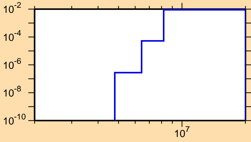
\sigma vs. E for ^{73}\text{As}(n,d)
