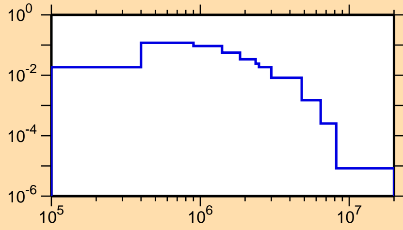
\sigma vs. E for ^{73}\text{As}(n,n_3)
