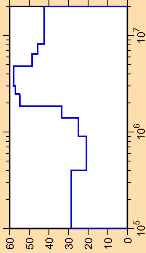
\Delta\sigma/\sigma vs. E for ^{73}\text{As}(n,n_3)
