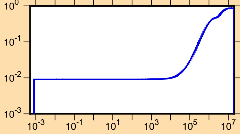
\mu vs. E for ^{74}\text{As}(\text{mt251})
