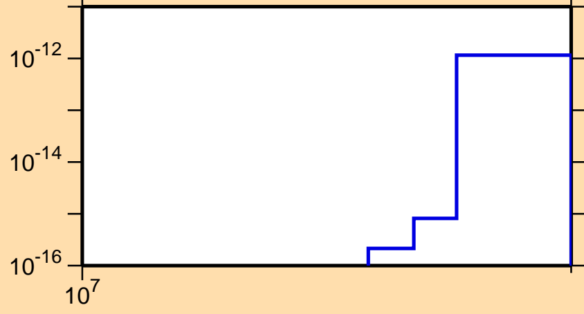
\sigma vs. E for ^{74}\text{As}(n,\text{pt})
