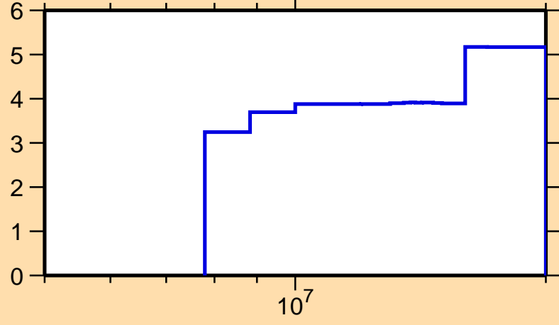
\Delta\sigma/\sigma vs. E for ^{74}\text{As}(n,\text{nonel.})
