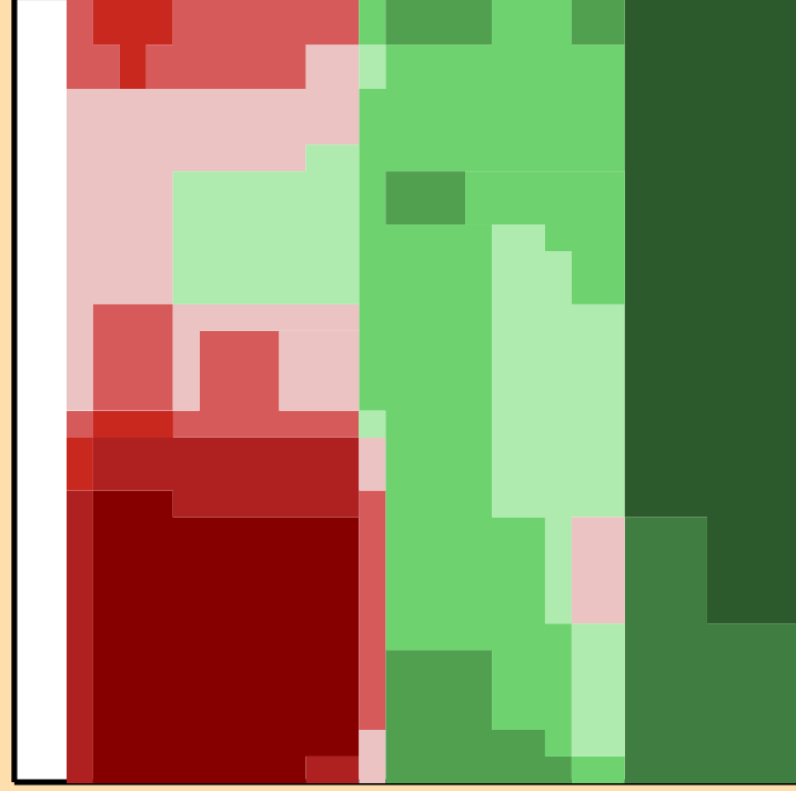
\Delta\sigma/\sigma vs. E for ^{74}\text{As}(n,ncont.)
