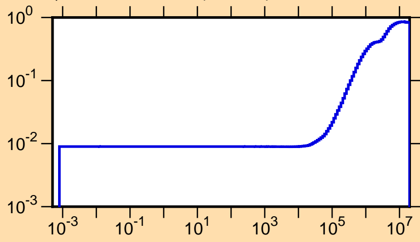
\mu vs. E for ^{75}\text{As}(\text{mt251})
