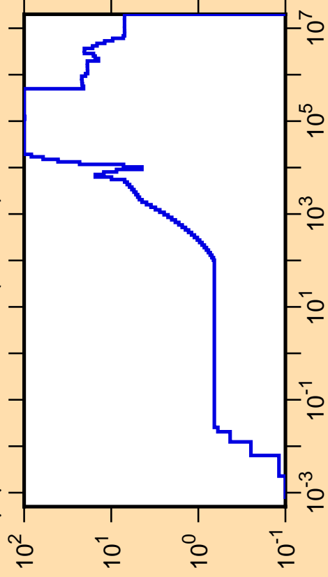
\Delta\mu/\mu vs. E for ^{75}\text{As}(\text{mt251})
