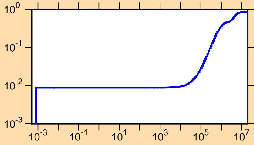
\mu vs. E for ^{76}\text{As}(\text{mt251})
