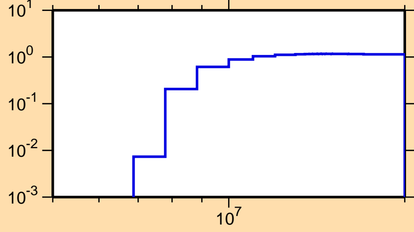
\sigma vs. E for ^{76}\text{As}(n,2n)
