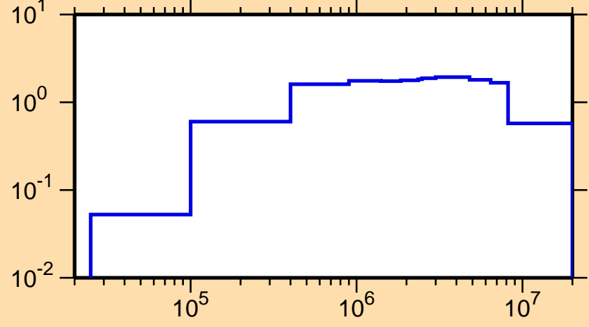
\sigma vs. E for ^{76}\text{As}(n,\text{inel.})
