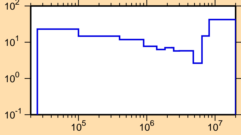
\Delta\sigma/\sigma vs. E for ^{76}\text{As}(n,\text{inel.})
