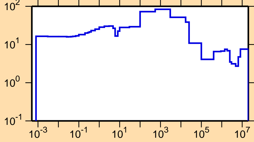
\Delta\sigma/\sigma vs. E for ^{76}\text{As}(n,\text{tot.})
