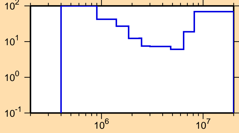
\Delta\sigma/\sigma vs. E for ^{76}\text{As}(n,ncont.)
