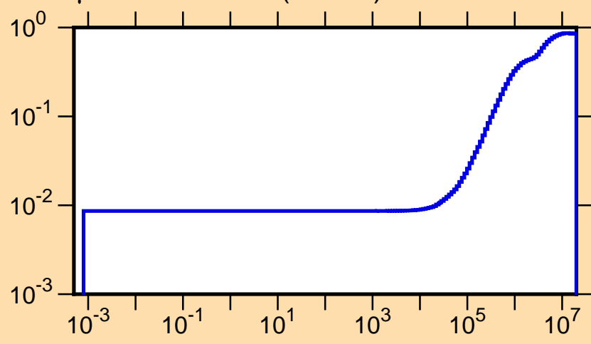
\mu vs. E for ^{78}\text{As}(\text{mt251})
