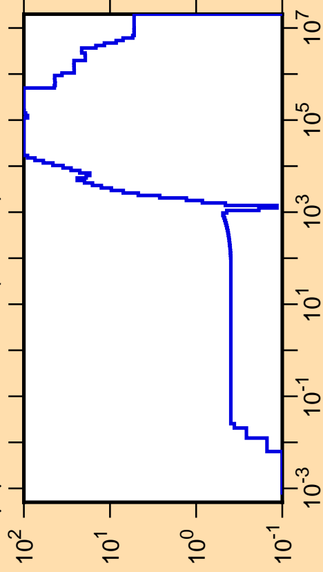
\Delta\mu/\mu vs. E for ^{78}\text{As}(\text{mt251})
