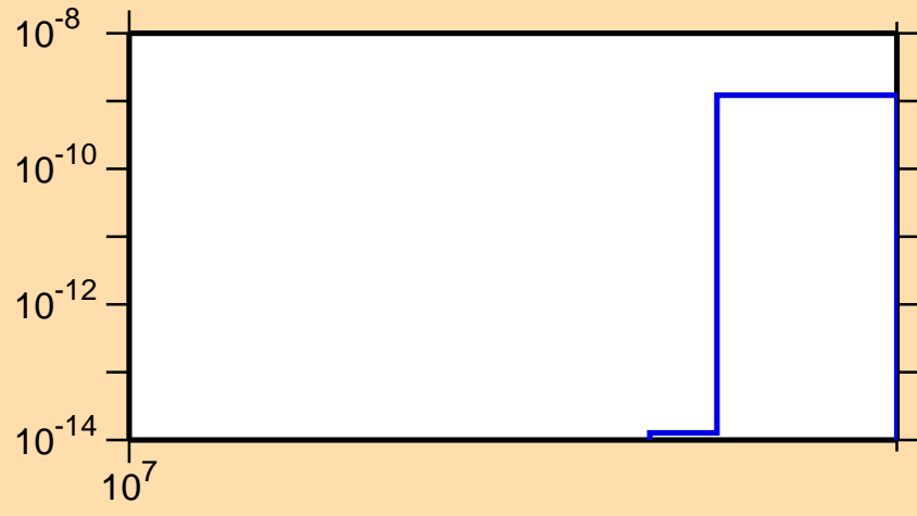
\sigma vs. E for ^{78}\text{As}(n,2n\alpha)
