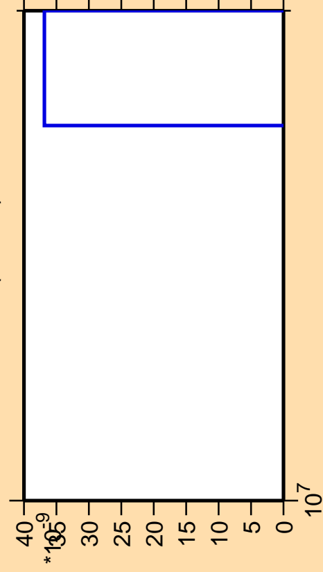
\Delta\sigma/\sigma vs. E for ^{78}\text{As} (mt 34)
