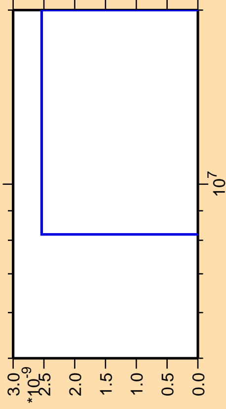
\Delta\sigma/\sigma vs. E for ^{78}\text{As}(n,pt)
