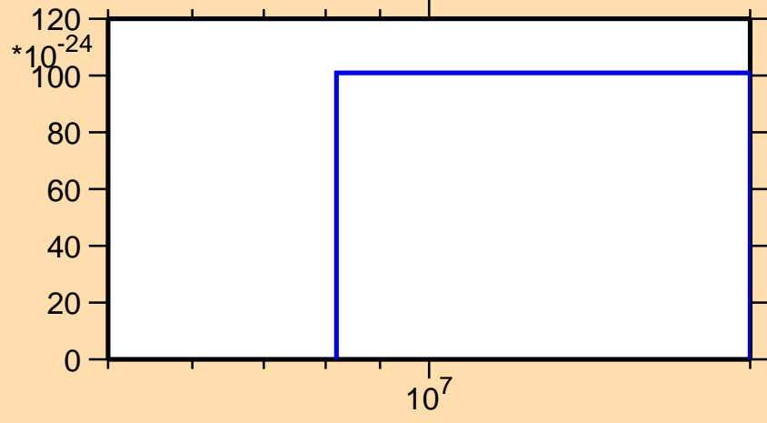
\sigma vs. E for ^{78}\text{As}(\text{mt } 34)
