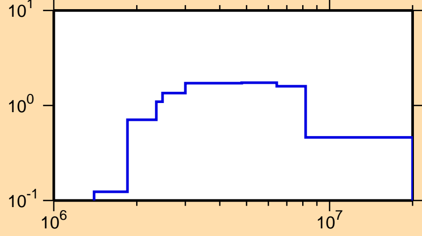
\sigma vs. E for ^{78}\text{As}(n,n\text{cont.})
