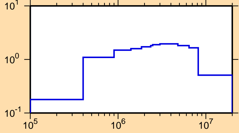
\sigma vs. E for ^{78}\text{As}(n,\text{inel.})
