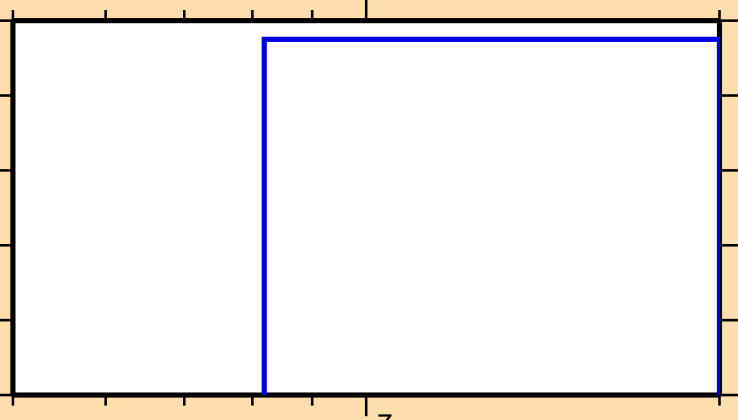
\sigma vs. E for ^{78}\text{As}(n,nt)
