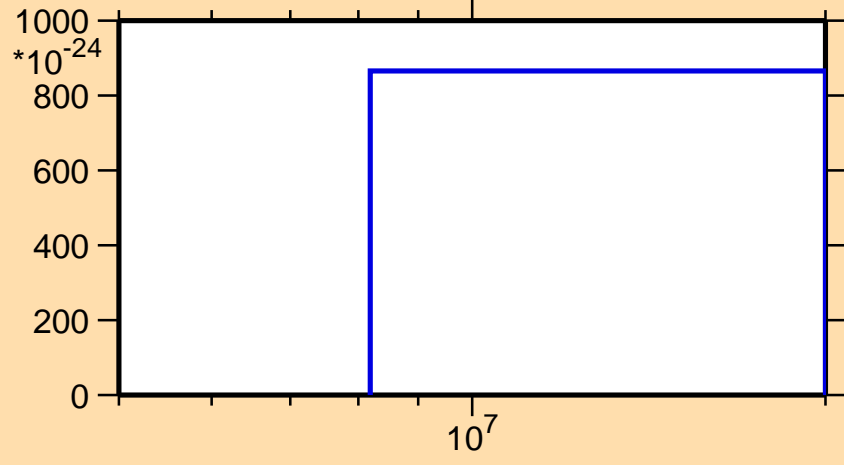
\sigma vs. E for ^{78}\text{As}(n,pt)
