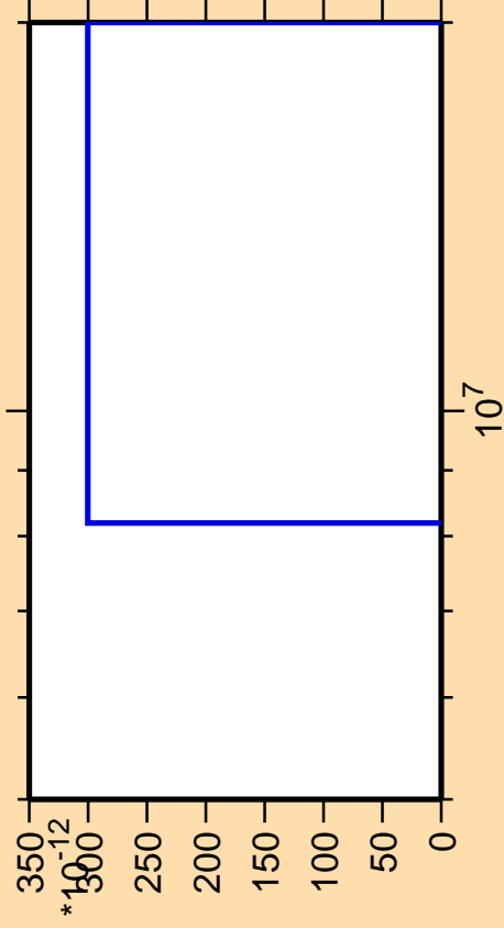
\Delta\sigma/\sigma vs. E for ^{78}\text{As}(\text{mt } 34)
