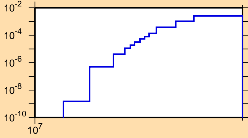
\sigma vs. E for ^{81}\text{As}(n,np)
