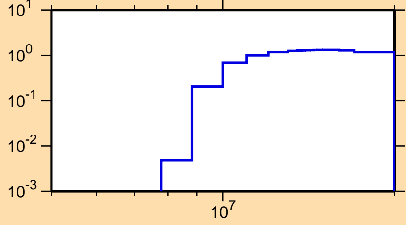
\sigma vs. E for ^{81}\text{As}(n,2n)
