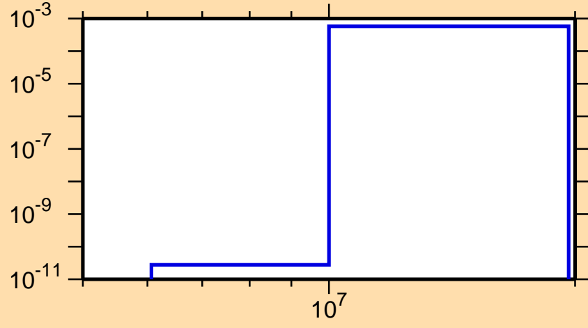
\sigma vs. E for ^{81}\text{As}(n,d)
