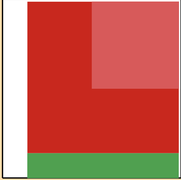
\Delta\sigma/\sigma vs. E for ^{81}\text{As}(n,2n)
