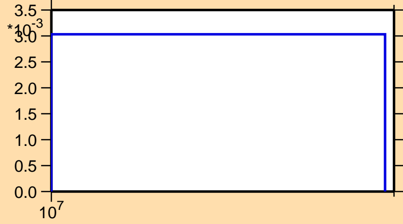
\sigma vs. E for ^{81}\text{As}(n,3n)
