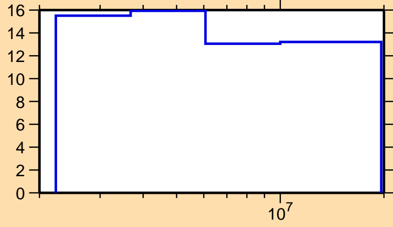
\Delta\sigma/\sigma vs. E for ^{81}\text{As}(n,n\text{onel.})
