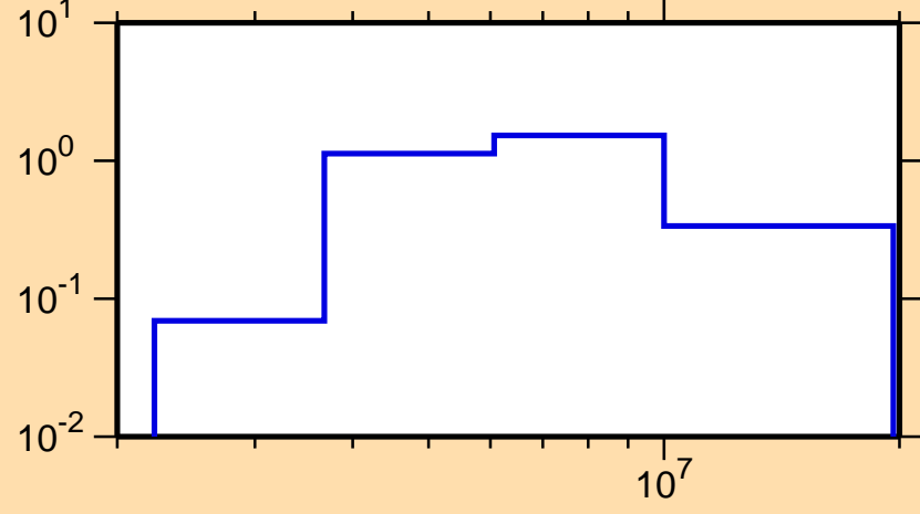
\sigma vs. E for ^{81}\text{As}(n,n\text{cont.})
