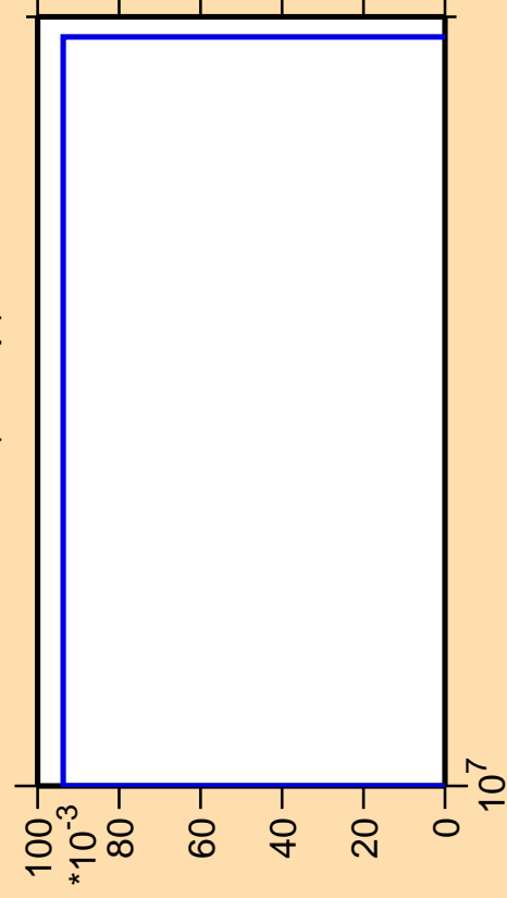
\Delta\sigma/\sigma vs. E for ^{81}\text{As}(n,2np)
