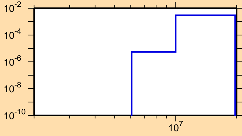
\sigma vs. E for ^{81}\text{As}(n,p)
