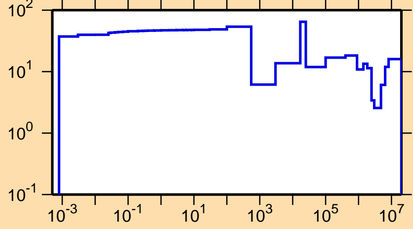
\Delta\sigma/\sigma vs. E for ^{81}\text{As}(n,\text{tot.})
