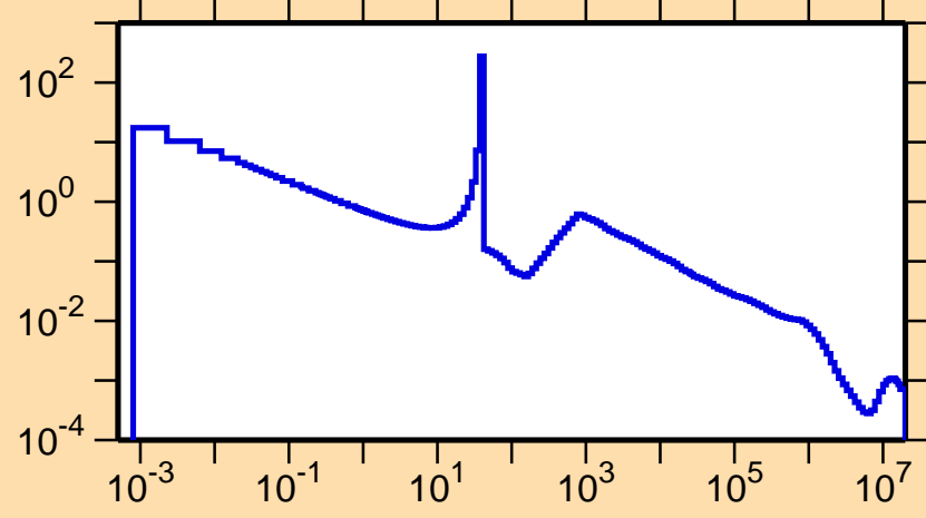
\sigma vs. E for ^{82}\text{As}(n,\gamma)
