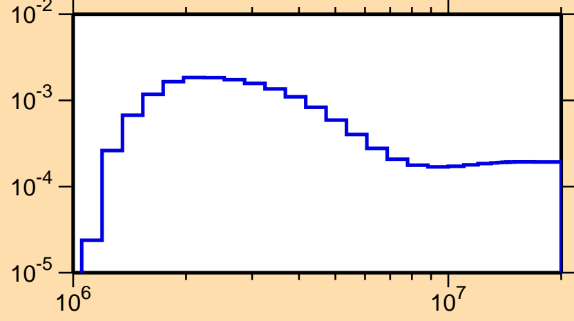
\sigma vs. E for ^{82}\text{As}(n,n_4)
