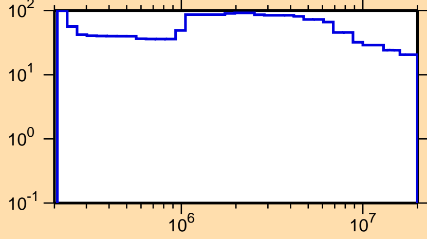
\Delta\sigma/\sigma vs. E for ^{82}\text{As}(n,n_1)
