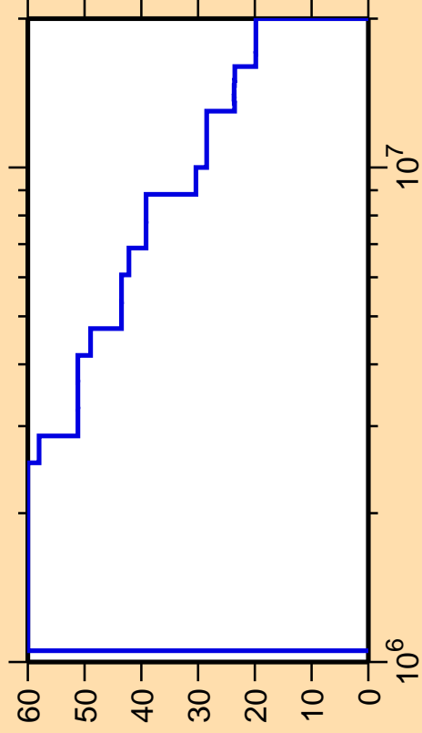
\Delta\sigma/\sigma vs. E for ^{82}\text{As}(n,n_3)
