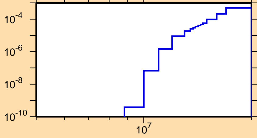
\sigma vs. E for ^{82}\text{As}(n,t)
