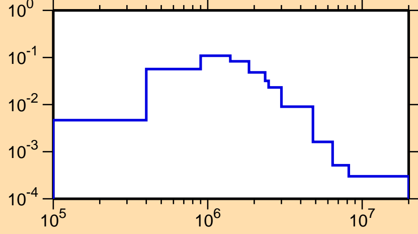
\sigma vs. E for ^{82}\text{As}(n,n_1)
