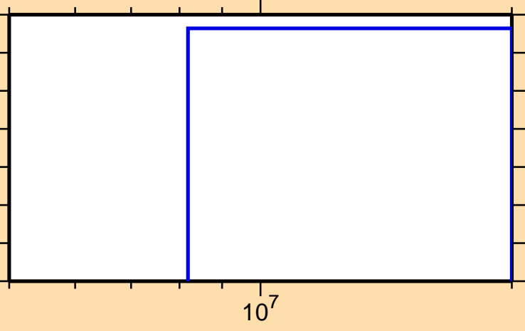
\sigma vs. E for ^{82}\text{As}(n,nt)
