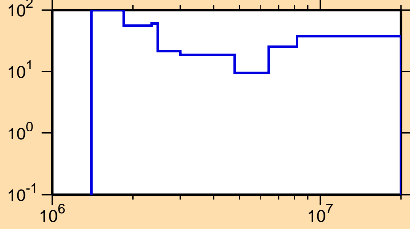
\Delta\sigma/\sigma vs. E for ^{82}\text{As}(n,ncont.)
