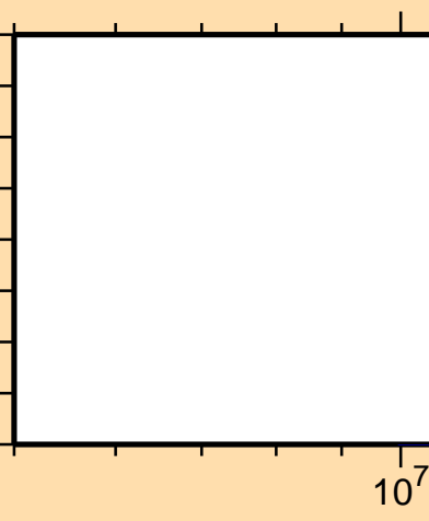
\sigma vs. E for ^{82}\text{As}(n,d)
