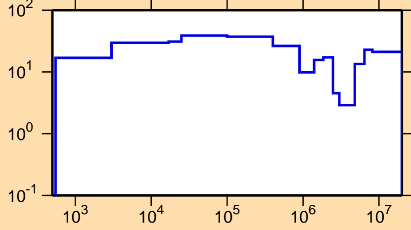
\Delta\sigma/\sigma vs. E for ^{82}\text{As}(n,\text{tot.})
