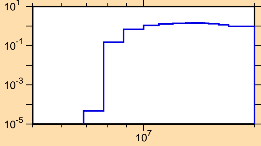
\sigma vs. E for ^{83}\text{As}(n,2n)
