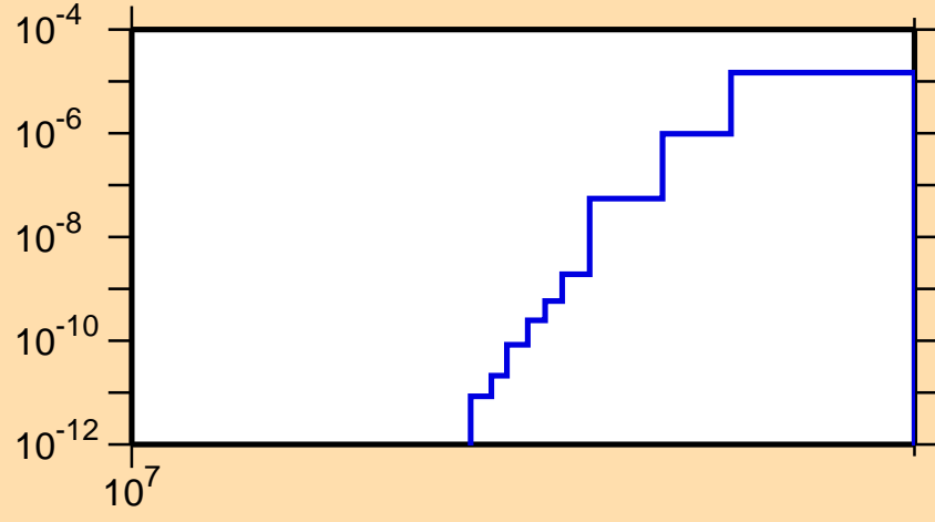
\sigma vs. E for ^{83}\text{As}(n,n\alpha)
