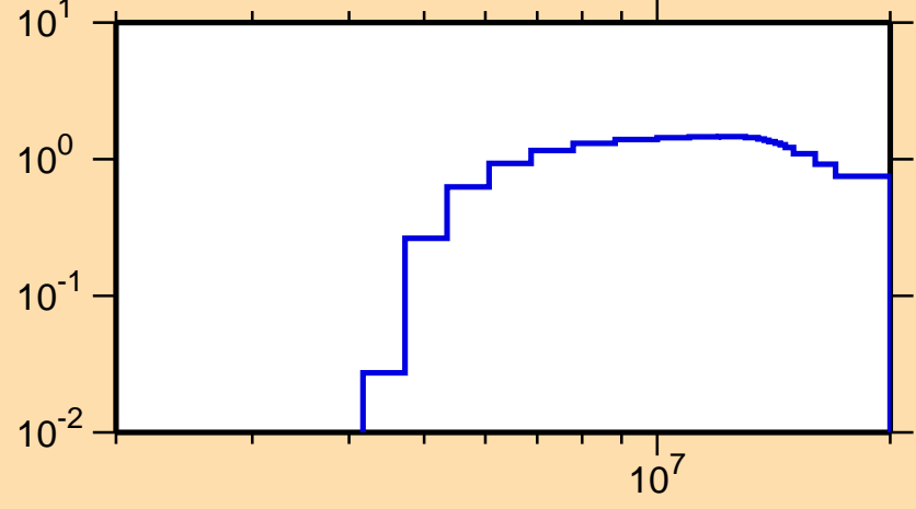
\sigma vs. E for ^{84}\text{As}(n,2n)
