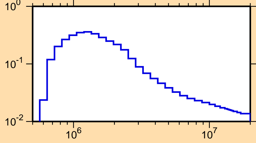
\sigma vs. E for ^{84}\text{As}(n,n_4)
