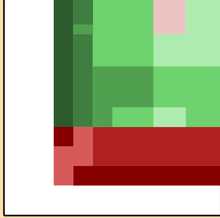
\Delta\sigma/\sigma vs. E for ^{84}\text{As}(n,p)
